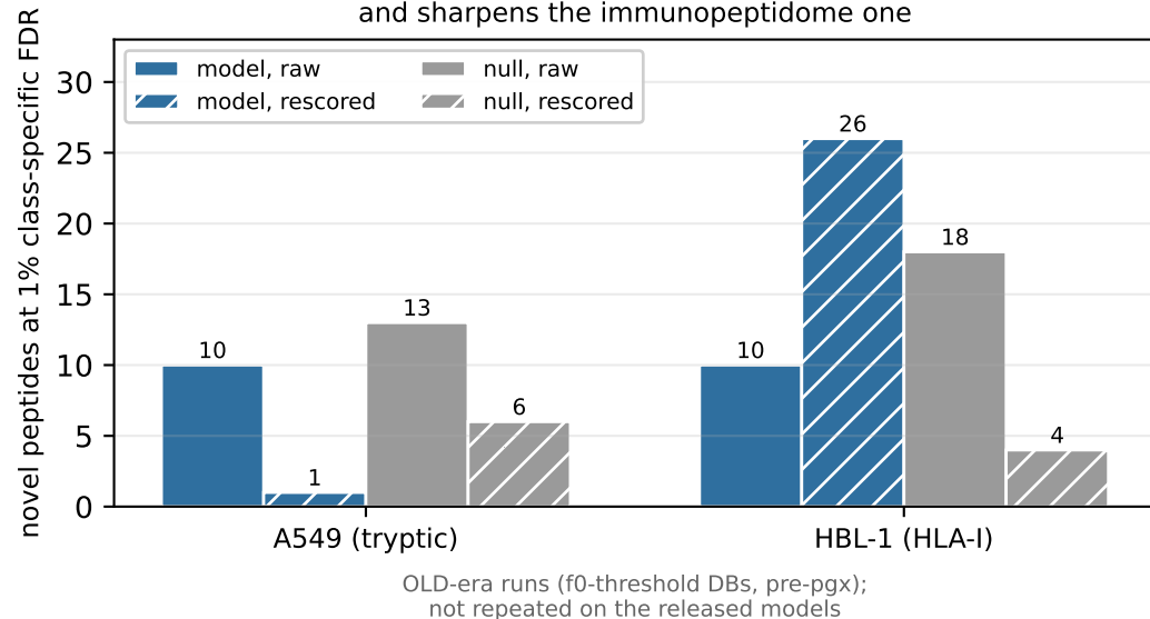
(b) the consequence: rescoring collapses the tryptic case and sharpens the immunopeptidome one
