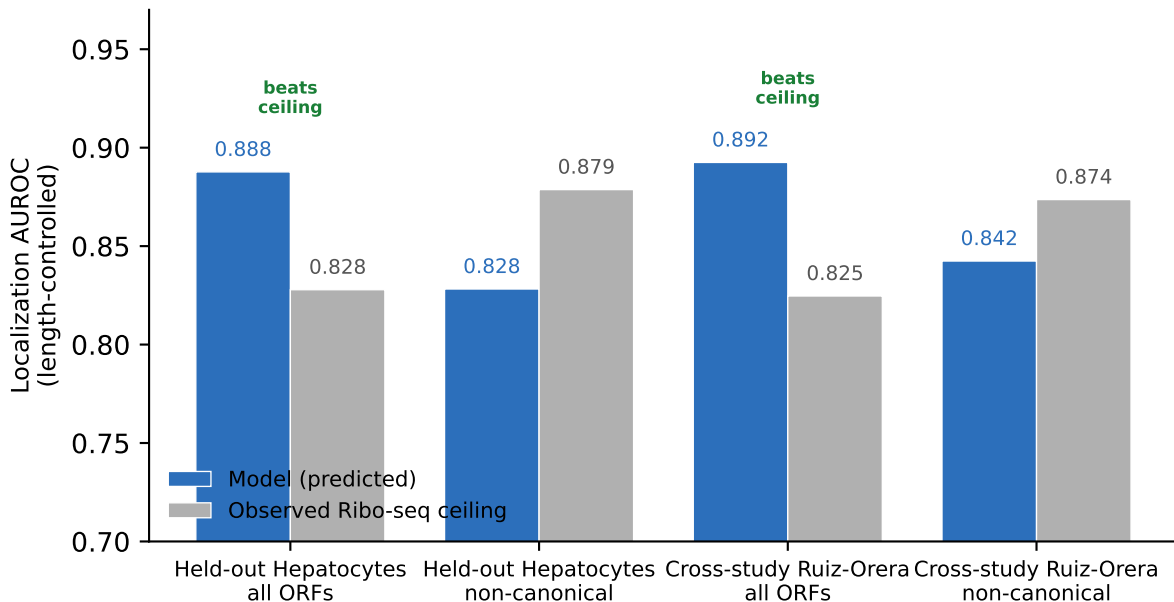
Predicted translation localization matches/beats the Ribo-seq ceiling
