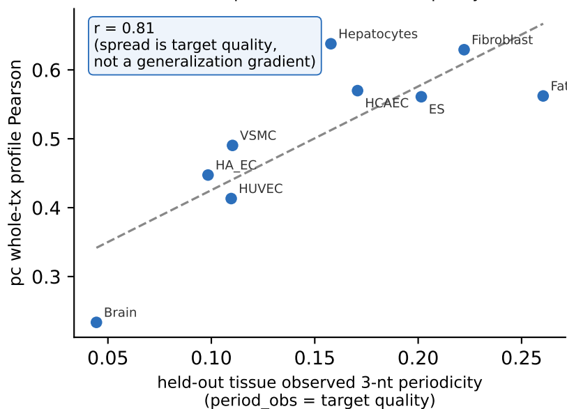
a Profile-Pearson spread = held-out data quality
