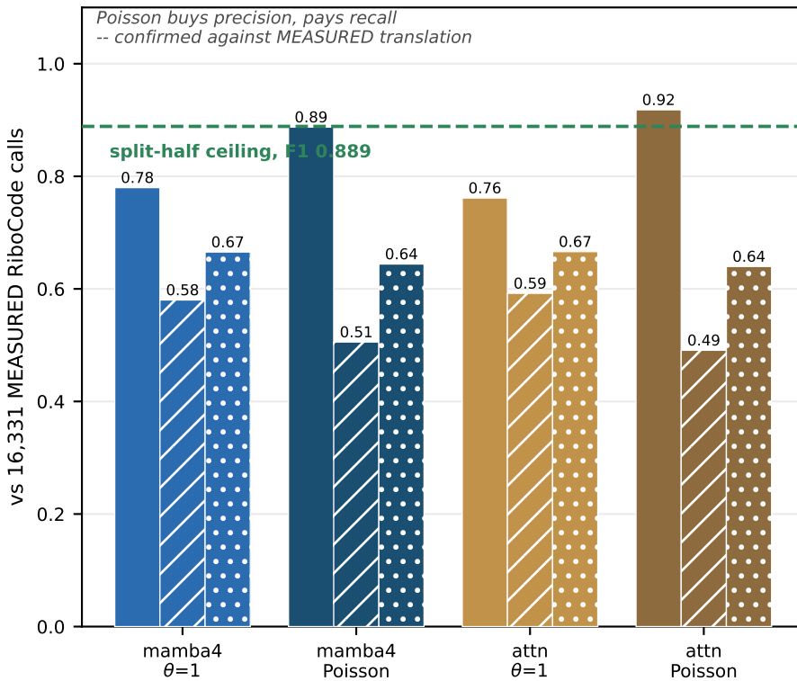
A Predicted vs measured (bars: precision / recall 1/2 / F1 1/3 )
