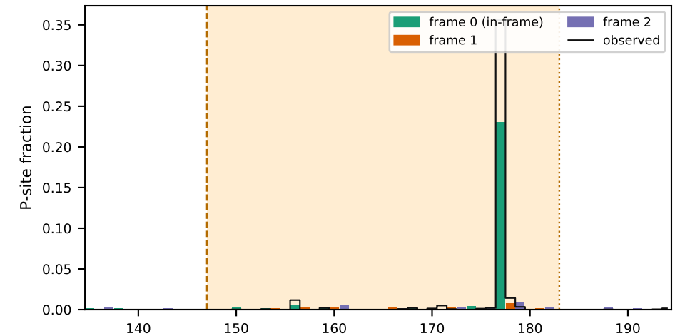
CDS zoom [137, 197] -- predicted P-sites colored by frame
