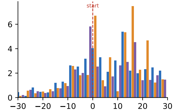
start-codon zoom (frame-colored)
