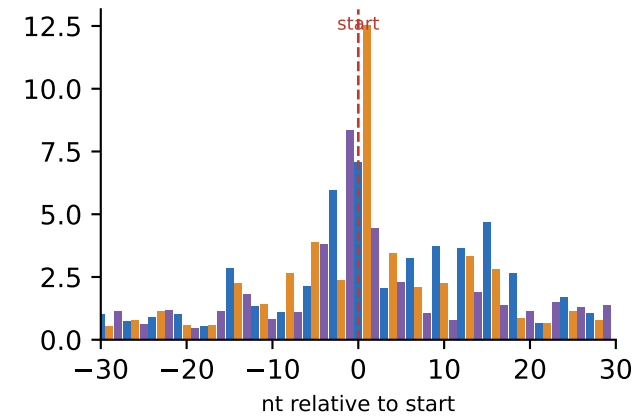
start-codon zoom (frame-colored)
