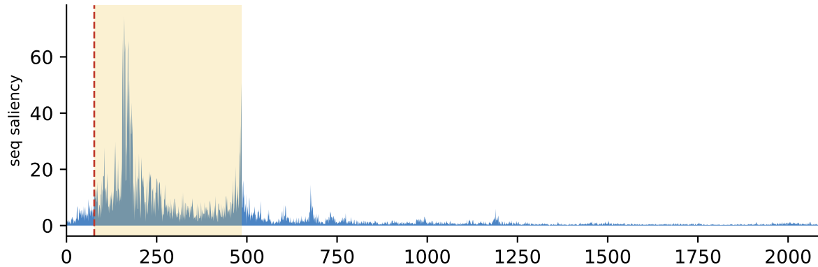
LINC02693 (lncRNA ORF, ENST00000647872.1)
