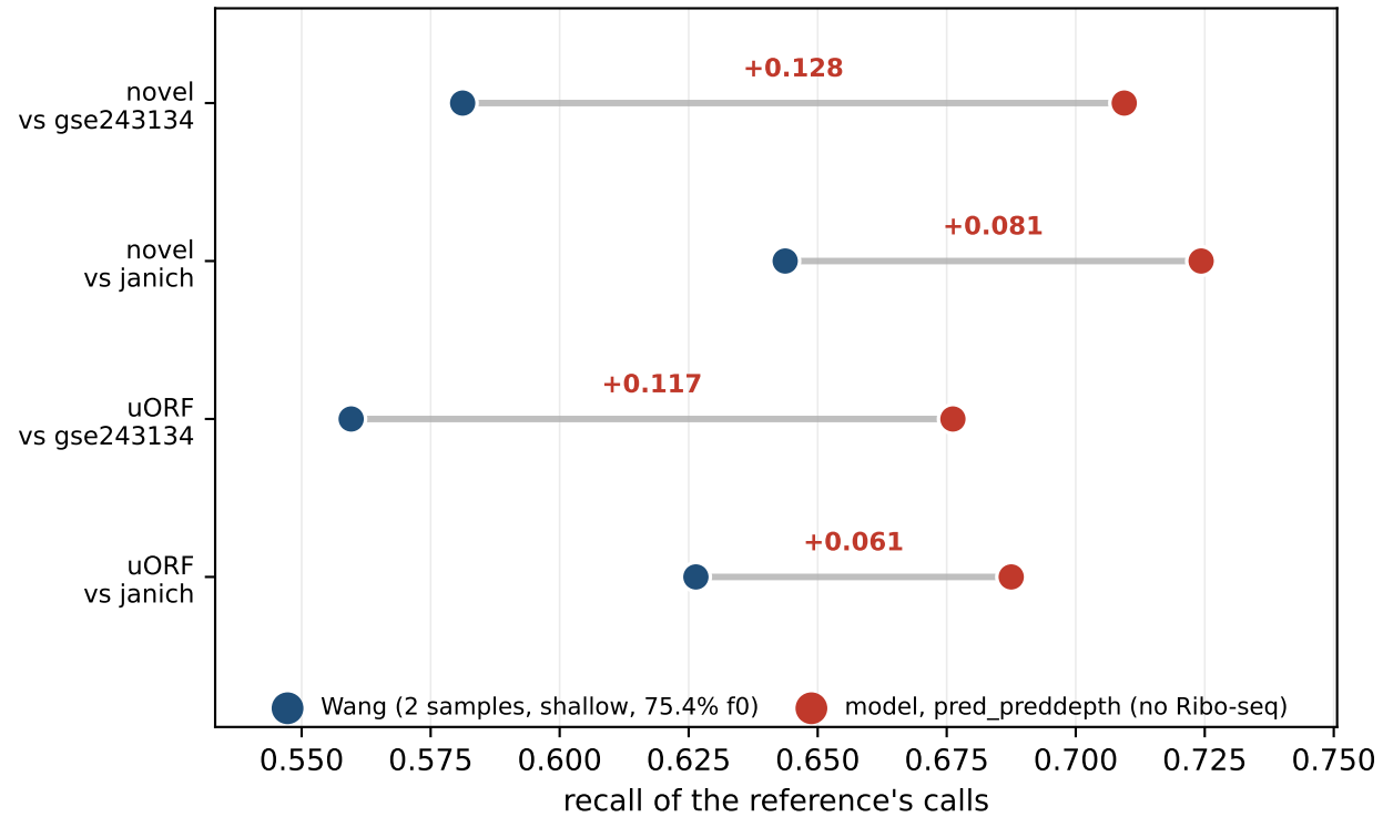
B Shallow experiment vs standalone model (no Ribo-seq)
