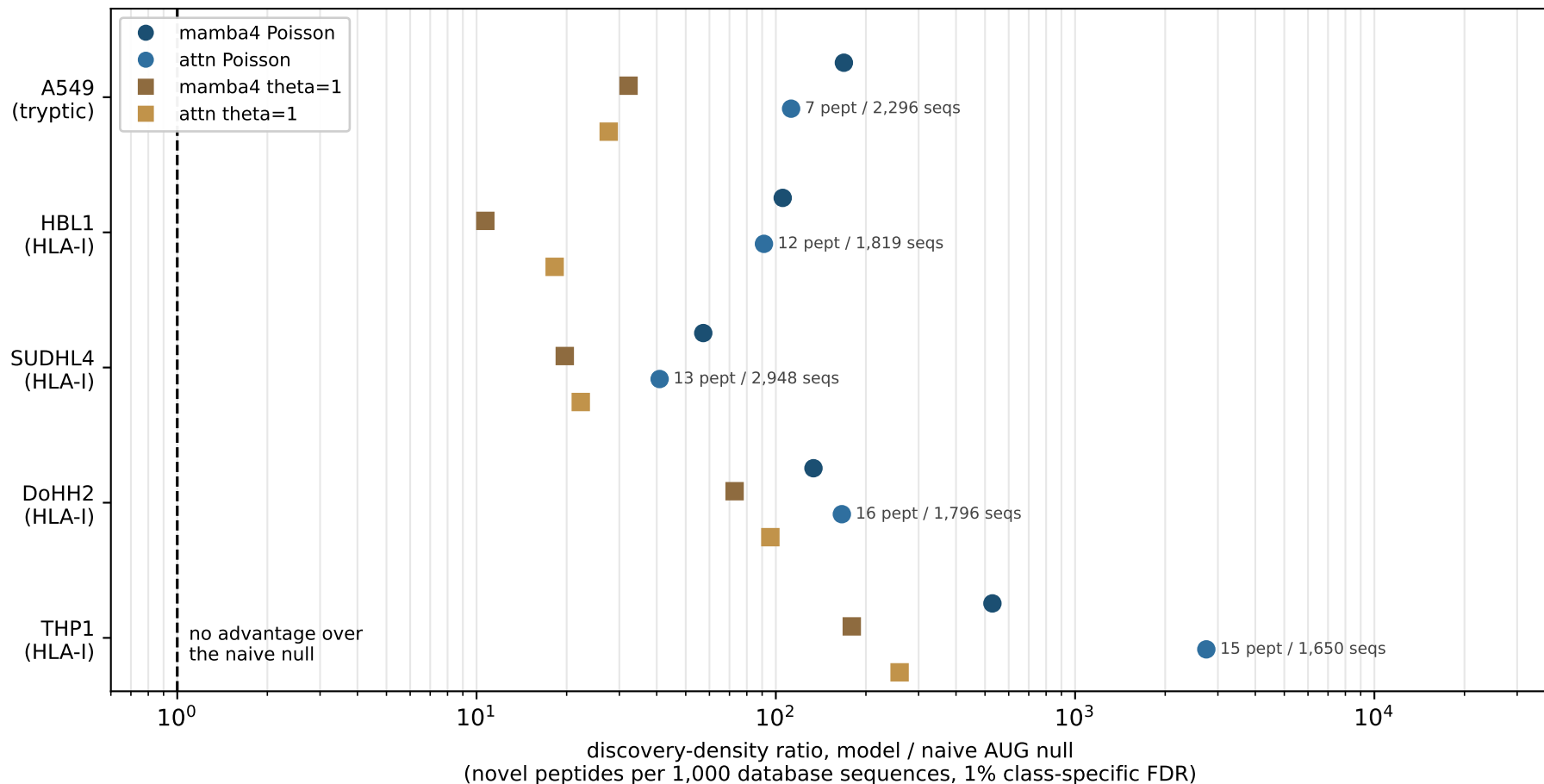
Fig 2b -- the model selects a denser search space than naive enumeration, reproducibly across 5 datasets and both released models
