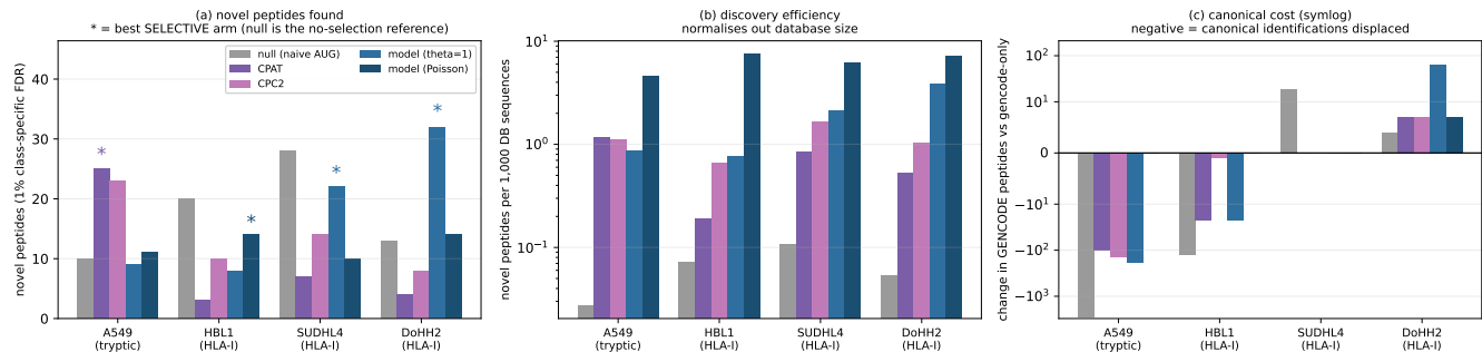
Predicting which ORFs to include keeps the DB compact: 2-3.4x higher discovery efficiency, far less CDS displacement, ~1/3 the decoy load vs the naive 3-frame null
