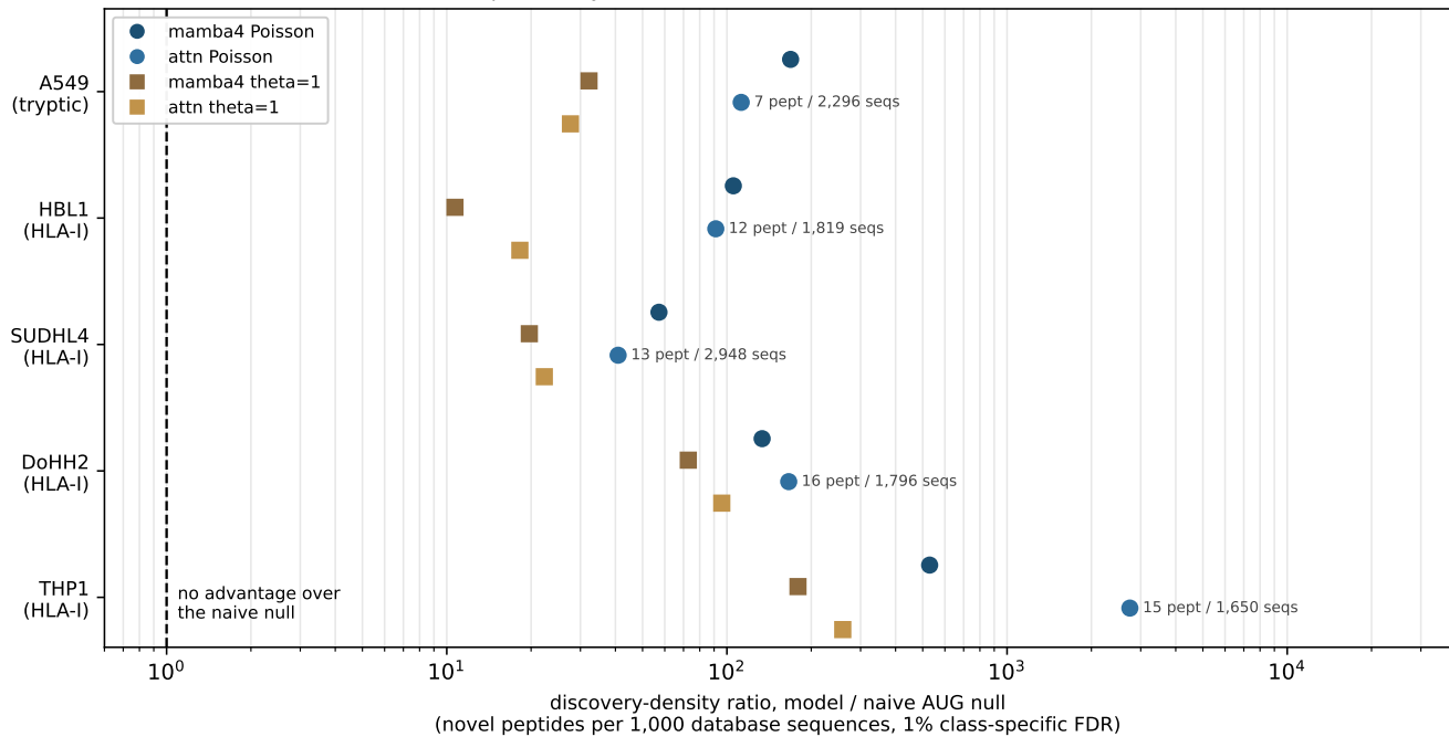
Fig 2b -- the model selects a denser search space than naive enumeration, reproducibly across 5 datasets and both released models
