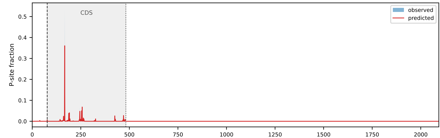
lncRNA | LINC02693 ENST00000647872.1 whole-transcript profile r = 0.694
