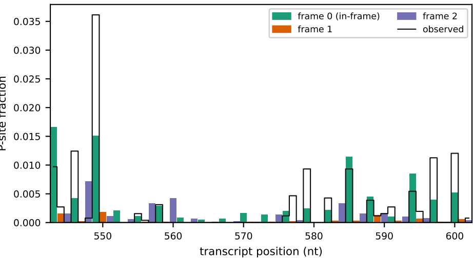
ORF zoom [543, 603] -- predicted P-sites colored by frame
