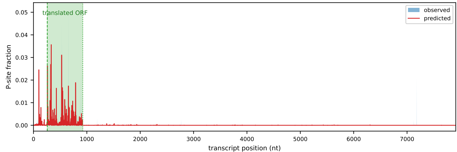
lncRNA | LINC02693 ENST00000647872.1 whole-transcript profile r = 0.694
