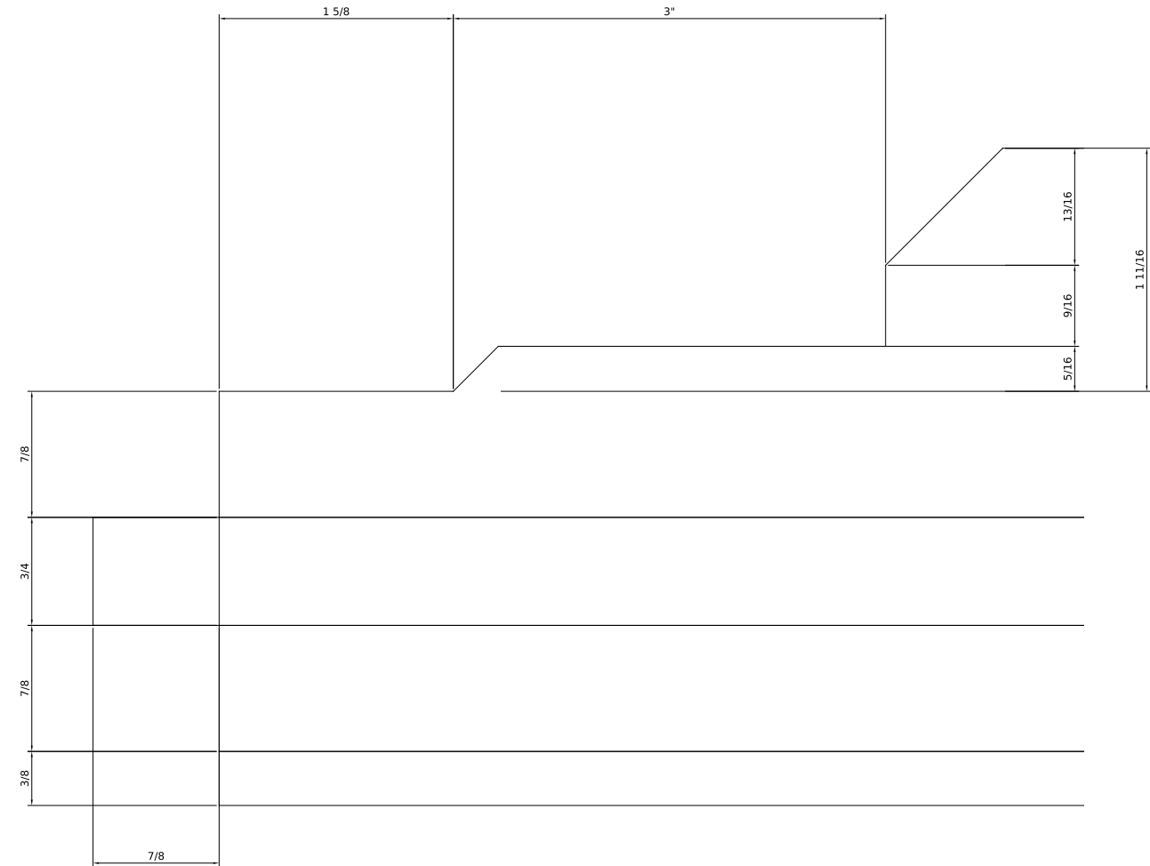
DETAIL A - LEFT END (SCALE 3:1)
