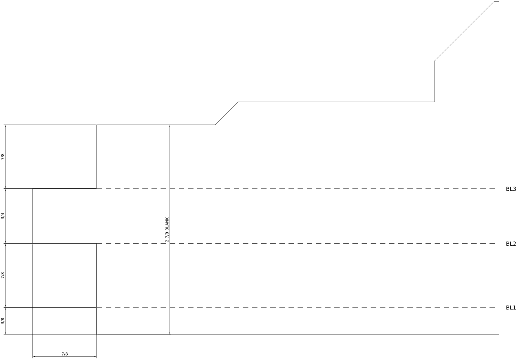
DETAIL - LEFT END (SCALE 4:1) right end is the same
