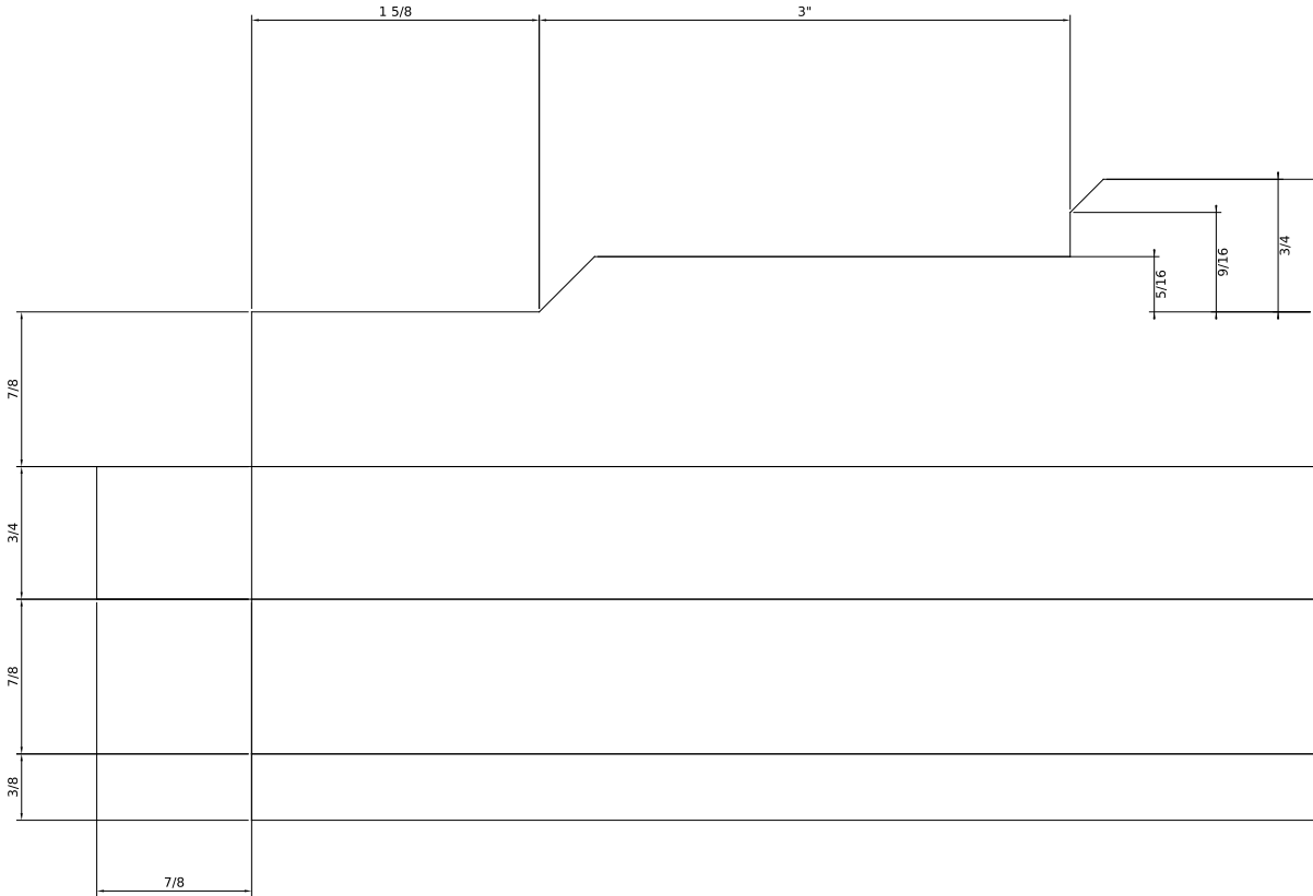
DETAIL A - LEFT END (SCALE 3:1)
