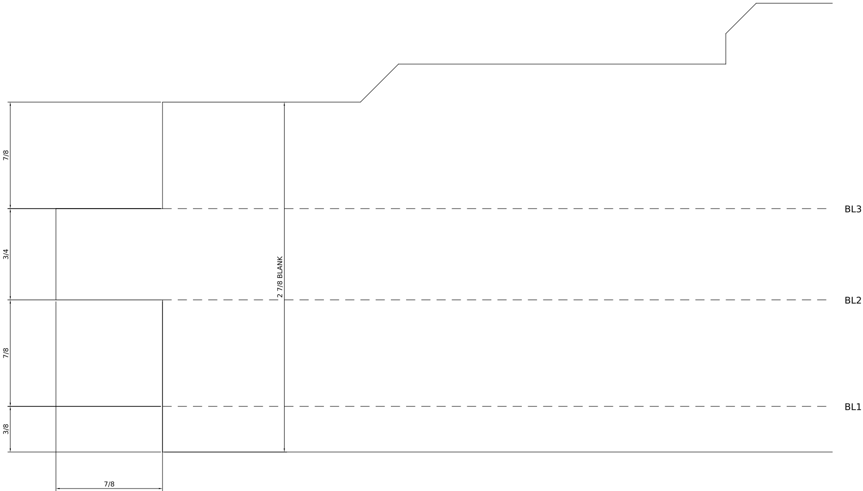
DETAIL - LEFT END (SCALE 4:1) right end is the same
