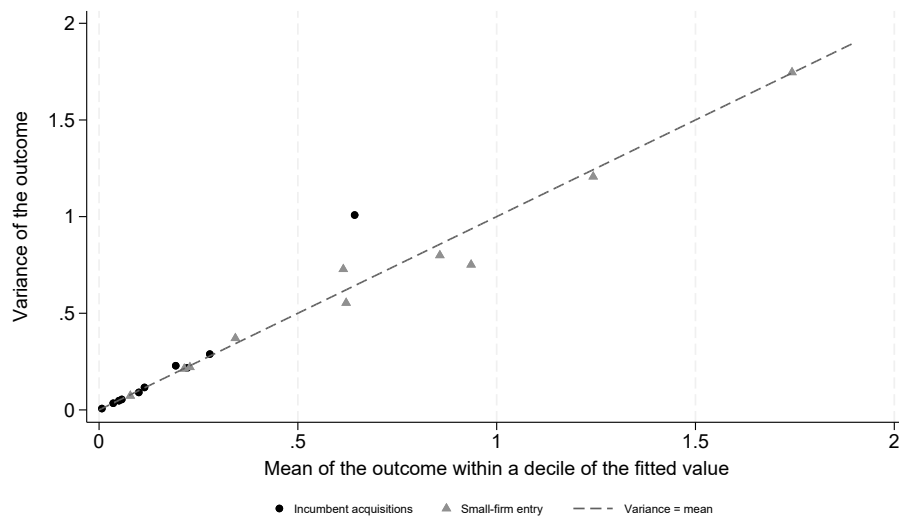
Figure 12: The variance of each count tracks its mean
