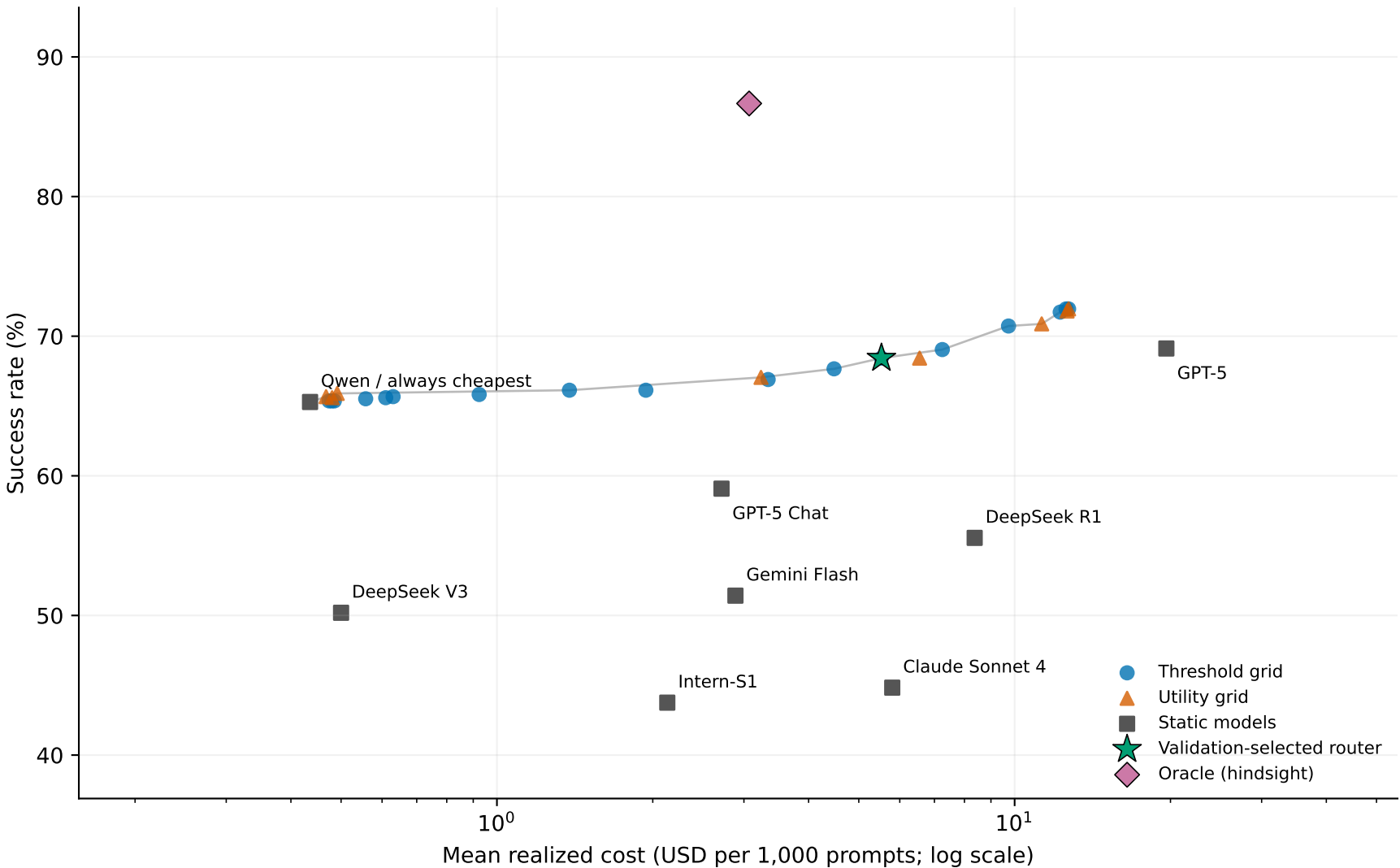
Standard Handcrafted: frozen test cost-quality points
