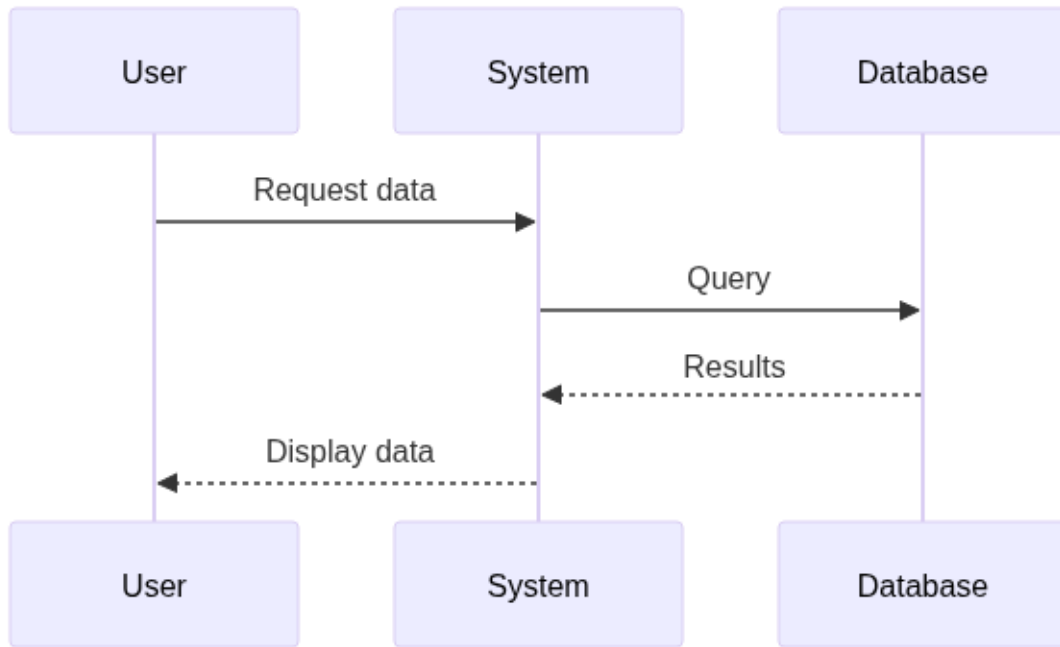
Figure 2: Mermaid Diagram
