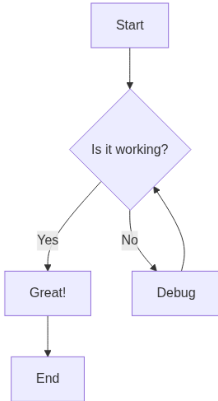
Figure 1: Mermaid Diagram
