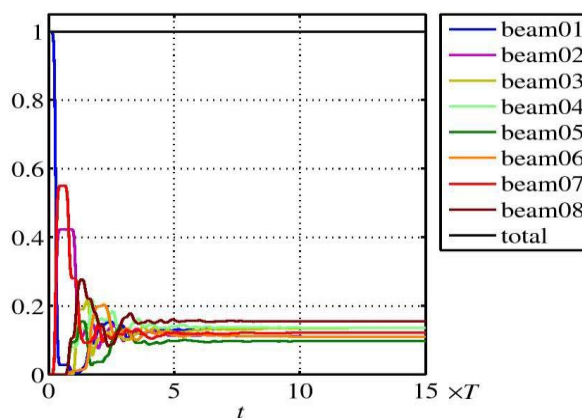
Figure 2-Evolution of the integrated vibrational energy.
