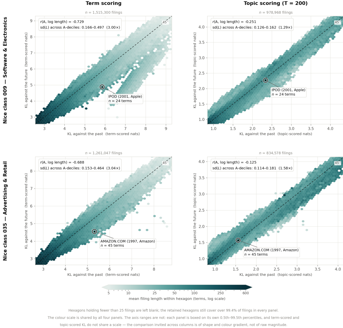
Figure 12: Mean filing length across the two axes, by representation and class. Hexagons holding fewer than 25 filings are blank; the retained hexagons cover over 99.4% of filings in every panel. The colour scale is shared across panels; the axis ranges are not, since term-scored and topic-scored KL do not share a scale, so the comparison invited across columns is of shape and colour gradient rather than of magnitude. Topic scoring returns a finite value for roughly 65% of filings, so the columns are not the same sample; the correlations quoted in Appendix A are re-estimated on the common subset and are substantially unchanged.
