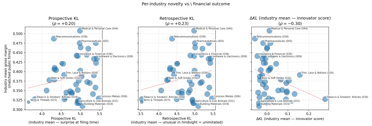
Figure 20: Each dot is one of the 45 NICE international classes; dot size is proportional to the number of matched public firms in the class. Left panel: industry-mean prospective KL (surprise at filing time) on the x -axis. Centre: industry-mean retrospective KL (remained-novel-in-hindsight). Right: industry-mean \Delta KL (imitated-innovator score). All three are plotted against industry-mean gross margin on the y -axis. Dashed lines are OLS fits, \rho is the Pearson correlation across the 45 industries.
