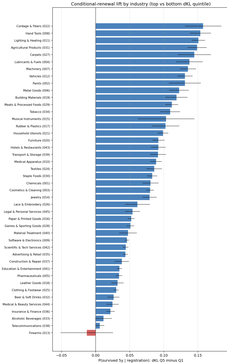
Figure 4: Conditional-renewal lift ( \Delta\text{KL} top minus bottom quintile, P(\text{alive at 5 years} \mid \text{registration}) ) for the 44 NICE classes with sufficient volume, with 95% intervals. Per-class figures and the summary table are in the repository under paper/results/per_industry/ .
