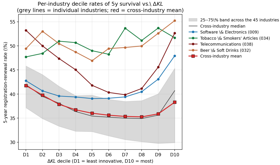
Figure 10: Per-decile 5y registration-renewal rate by \Delta KL decile. Each grey line is one of the 45 NICE industries; red is the cross-industry mean. The U-shape is visible in nearly every industry.
