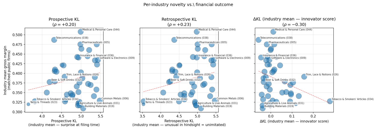
Figure 11: Each dot is one of the 45 NICE international classes; dot size is proportional to the number of matched public firms in the class. Left panel: industry-mean prospective KL (surprise at filing time) on the x -axis. Centre: industry-mean retrospective KL (remained-novel-in-hindsight). Right: industry-mean \Delta KL (imitated-innovator score). All three are plotted against industry-mean gross margin on the y -axis. Dashed lines are OLS fits, \rho is the Pearson correlation across the 45 industries.
