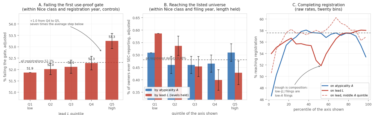
Figure 2: Quintile profiles for the three outcomes. A : the share of registrations failing the first use-proof gate, by lead quintile, adjusted within Nice class and registration year with the drafting and filer controls of Table 3; the dashed line is the rate for all registrations. The profile rises gently and monotonically through the fourth quintile and then steps up: about seven tenths of the top-to-bottom gap is the single step from the fourth quintile to the fifth, seven times the average step below it. A gradient is present, but the step at the top dominates it, and the text reports top-versus-bottom contrasts for that reason. B : the share of first-time filers whose owner ever reaches SEC reporting, by quintile of atypicality and of lead, adjusted within Nice class and filing year with description length held; flat in atypicality, and falling in lead through the fourth quintile once the levels are controlled. Whiskers in A and B are 95% intervals on the difference from the bottom quintile. C : raw registration rates for debut filings in twenty bins — an inverse-U on atypicality, and on lead a trough just above the median that is compositional, absent once atypicality is held in its middle fifth (dashed). Horizontal line at the pooled rate.
