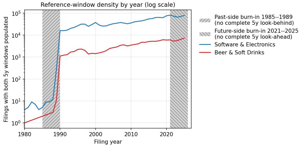
Figure 11: Reference-window density by year on log scale. Hatched regions are the past-side and future-side burn-in zones where the 5-year window is incomplete. The windows determine only how surprising a filing’s language is — its score at the filing date. The outcome the score is tested against is read separately and later: whether the registration survived the use-proof gate, decided at registration age six to seven, which is why the score is interpretable from 1995 but the gate sample ends with the 2018 cohort.
