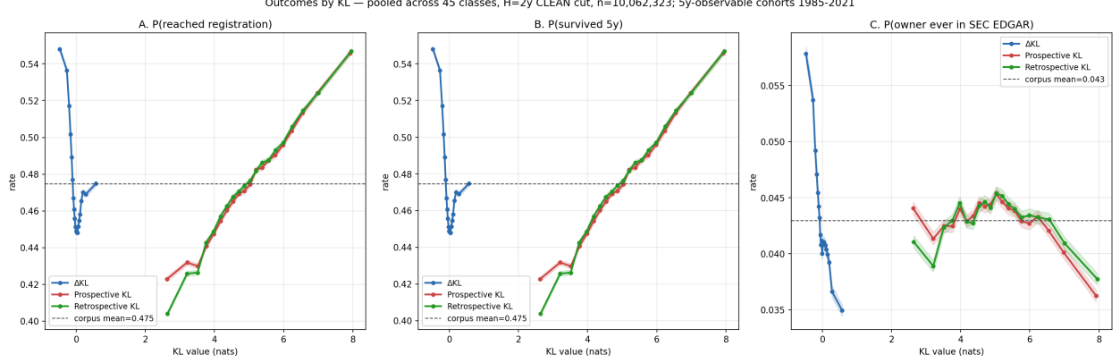
Figure 10: Three outcomes by \Delta KL , KL_{\text{pros}} , and KL_{\text{retr}} bin, pooled across all 45 NICE classes ( n=10.1\text{M} clean H=2\text{y} filings, 1985–2021). Each panel is one outcome: (A) P(\text{reached registration}) — examiner approval; (B) P(\text{survived } 5\text{y conditional on reaching registration}) ; (C) P(\text{owner ever in SEC EDGAR}) . The supported finding is that \Delta KL (blue) is U-shaped under every outcome definition — both flux extremes outperform the flux-neutral middle by 5–10 percentage points on post-registration survival — while KL_{\text{pros}} and KL_{\text{retr}} individually are monotone-increasing on examiner approval and only become U-shaped under the strict post-registration mortality criterion. The U on \Delta KL is the headline; the U on the components is an artefact of layering the maintenance-lapse filter onto the approval-monotone regime.
