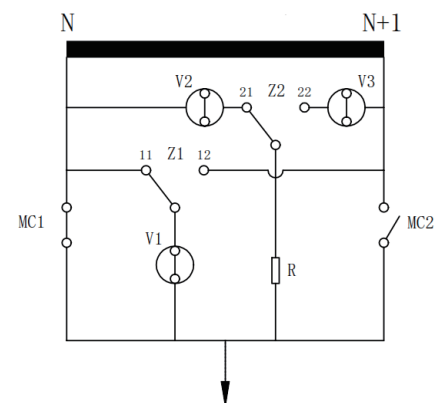
Electrical Topology Diagram
