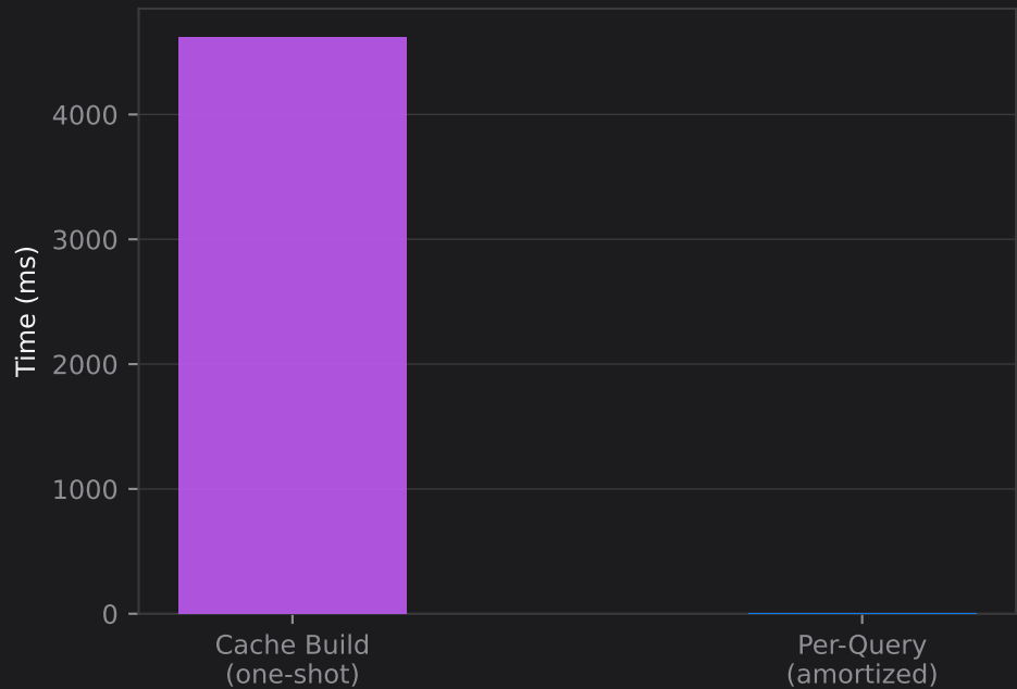
Cache Build: 4617.0 ms | Amortized: 10.17 \mu s/artifact
