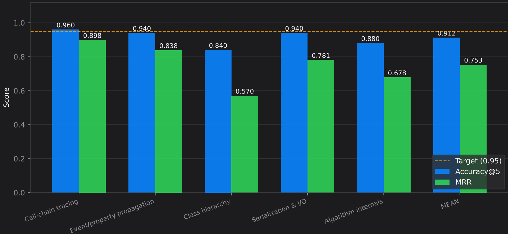
Accuracy@5 and MRR per Seed Dataset
