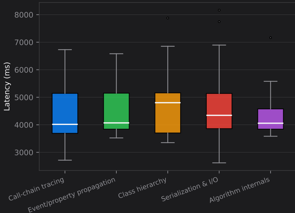
Latency by Seed Dataset
