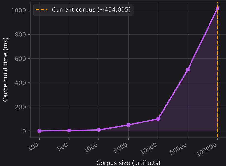
Amortized Numpy Cache Build Time vs Corpus Size
