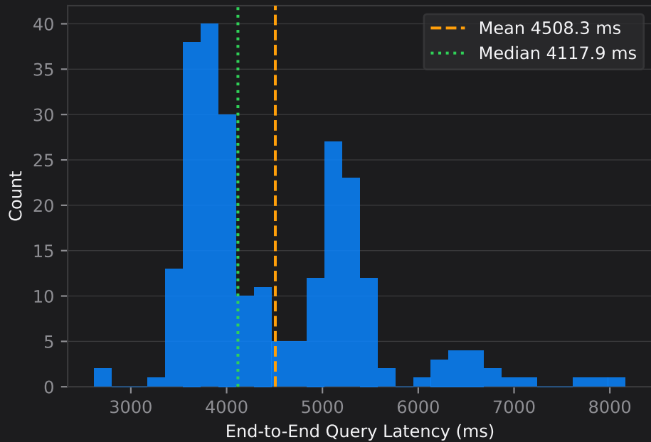
Query Latency Distribution (n=250)
