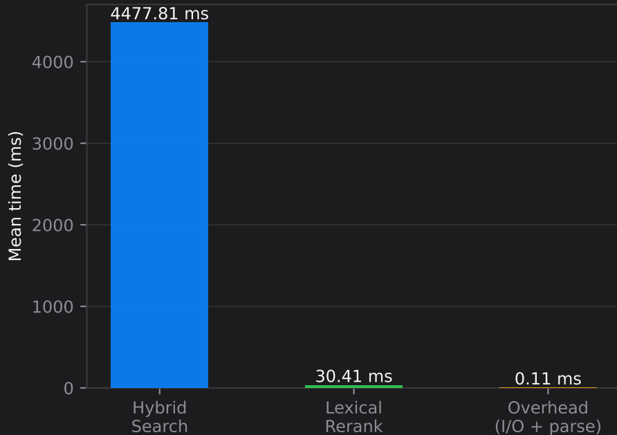
Mean Retrieval Stage Breakdown
