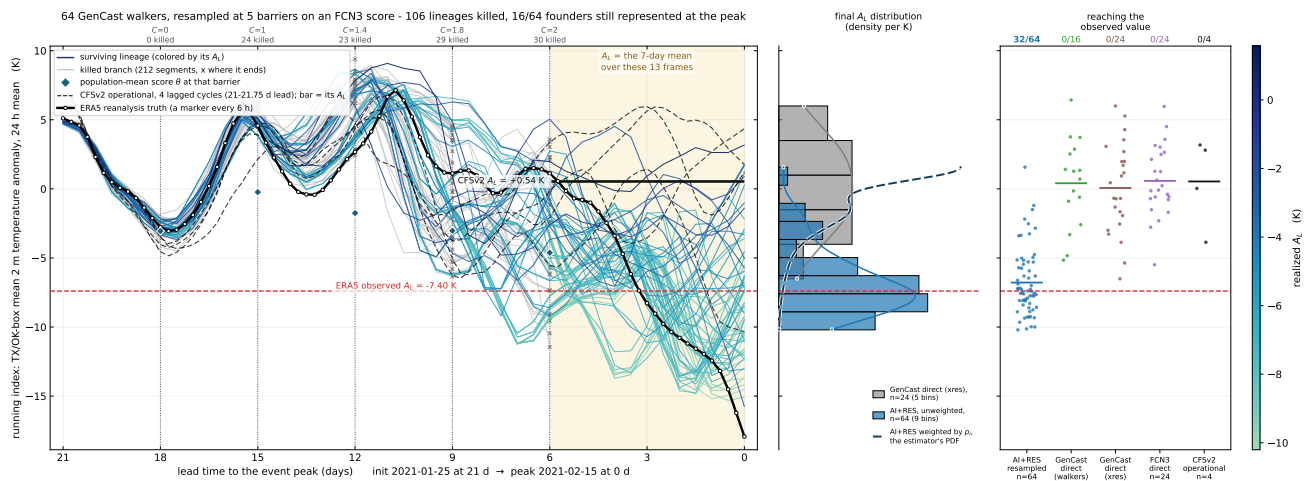
Figure A2: Winter Storm Uri, February 2021, over the Texas and Oklahoma region. The sign of the score is reversed for a cold event, so the method clones the coldest trajectories rather than the warmest. The schedule is otherwise the one used for the heat waves and was not retuned. Observed -7.40 K, reached by 32 of 64 trajectories, coldest -10.20 K. None of 24 direct GenCast members, 16 free-running trajectories or 24 direct FourCastNet 3 members reaches it.
