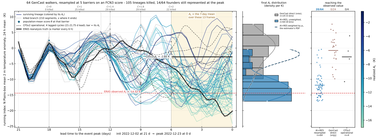
Figure A3: Winter Storm Elliott, December 2022, over the northern Plains region. This is the deepest cold target in the set relative to the forecast model's own spread. Observed -14.42 K, reached by 20 of 64 trajectories, coldest -17.04 K. The coldest direct member stops 4.6 K short at -9.83 K.
