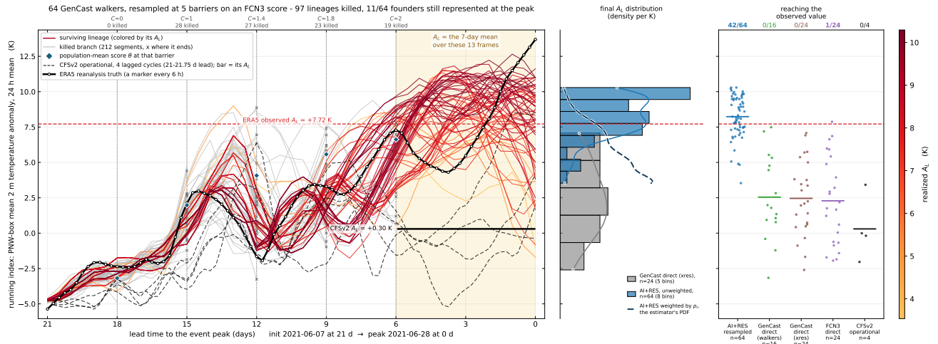
Figure C1: The 2021 Pacific Northwest heat dome, 64 trajectories, forecast from 21 days out. Left. Each line is one trajectory, plotted as its running regional temperature anomaly against time. Grey lines were discarded at a resampling step. Coloured lines survived to the event and are shaded by the value they reached. The dotted verticals are the five resampling steps, labelled by how hard the population was pushed and by how many trajectories were discarded. The blue diamonds are the population-average score. The shaded band on the right is the week the forecast is scored over. The black line with markers is the observed weather. The black dashed curves are the four CFSv2 operational cycles at the same lead, with their average drawn as a bar across the scored week. Middle. The distribution of final values for the 24-member direct GenCast ensemble in grey, for the AI+RES population in blue, and for the weighted estimate as a dashed line. Right. Where each method's members landed, with the number that reached the observed value printed above each column. Observed +7.72 K, reached by 42 of 64 trajectories, most extreme +10.29 K. The direct ensemble reaches it with none of 24 and stops at +7.08 K.
