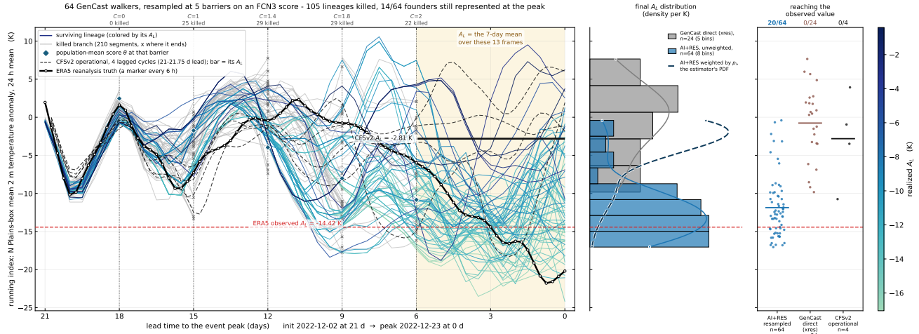
Figure A6: Winter Storm Elliott, December 2022, over the northern Plains region. This is the deepest cold target in the set relative to the forecast model's own spread. Observed -14.42 K, reached by 20 of 64 trajectories, coldest -17.04 K. The coldest direct member stops 4.6 K short at -9.83 K.
