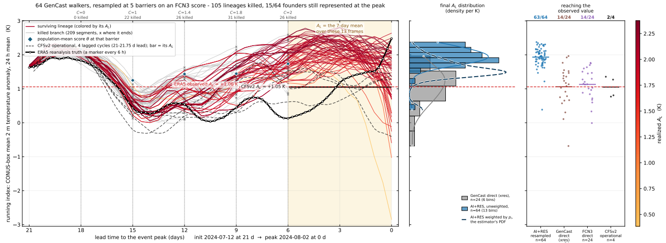
Figure A8: The CONUS-wide warm week of August 2024, the first mild control. Observed +1.06 K, reached by 63 of 64 trajectories, most extreme +2.37 K. Direct GenCast reaches it with 14 of 24 members, direct FourCastNet 3 with 14 of 24, and CFSv2 with 2 of 4 cycles. Where every method resolves the event, the weighted AI+RES estimate agrees with the direct count within sampling error (Section 5, item 2).
