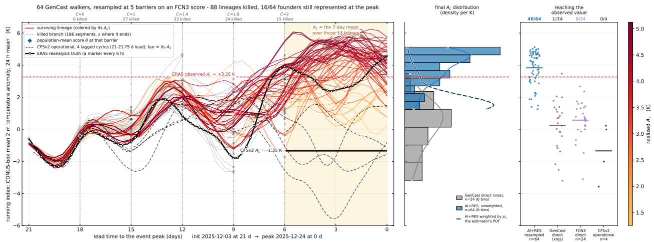
Figure A5: The CONUS-wide warm week of December 2025. This is the one extreme in Table 1 that direct sampling reaches, with 1 of 24 members at +3.46 K. Observed +3.26 K, reached by 46 of 64 trajectories, most extreme +5.12 K. The direct 24-member FourCastNet 3 ensemble at 21 days reaches it with none.
