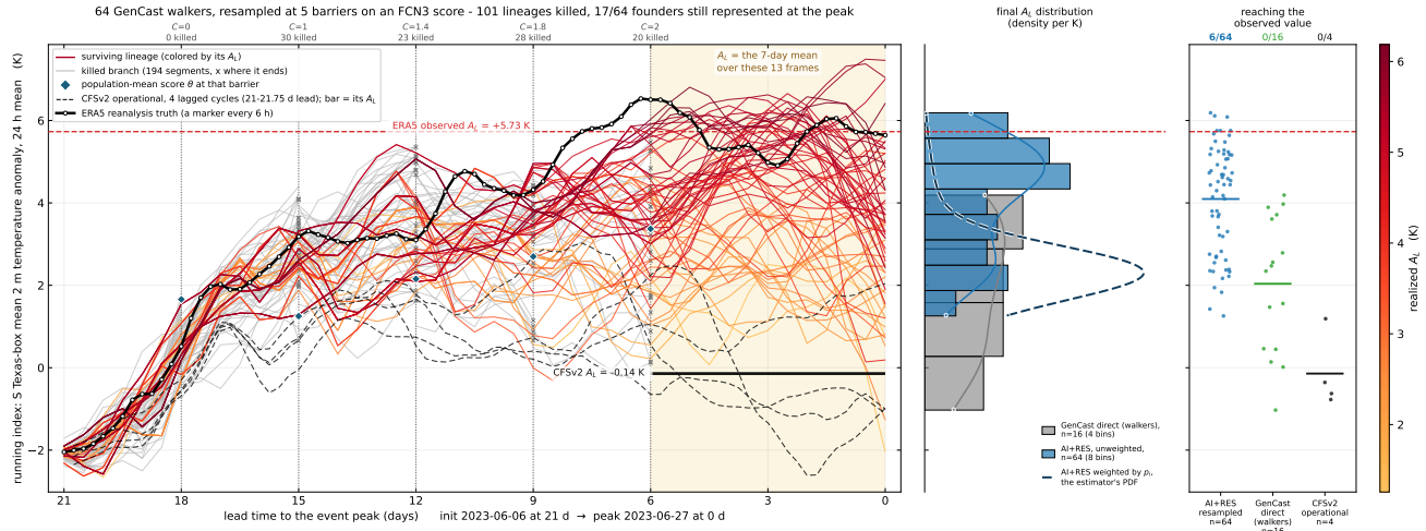
Figure A2: The June 2023 S. Texas heat dome, the event with no analogue in the 1959 to 2022 record. The direct column is the 16 free-running GenCast trajectories at 21 days, the only direct baseline for this region (Section 3). Observed +5.73 K, reached by 6 of 64 trajectories, most extreme +6.19 K. None of the 16 direct trajectories reaches it, the closest stopping at +4.19 K.
