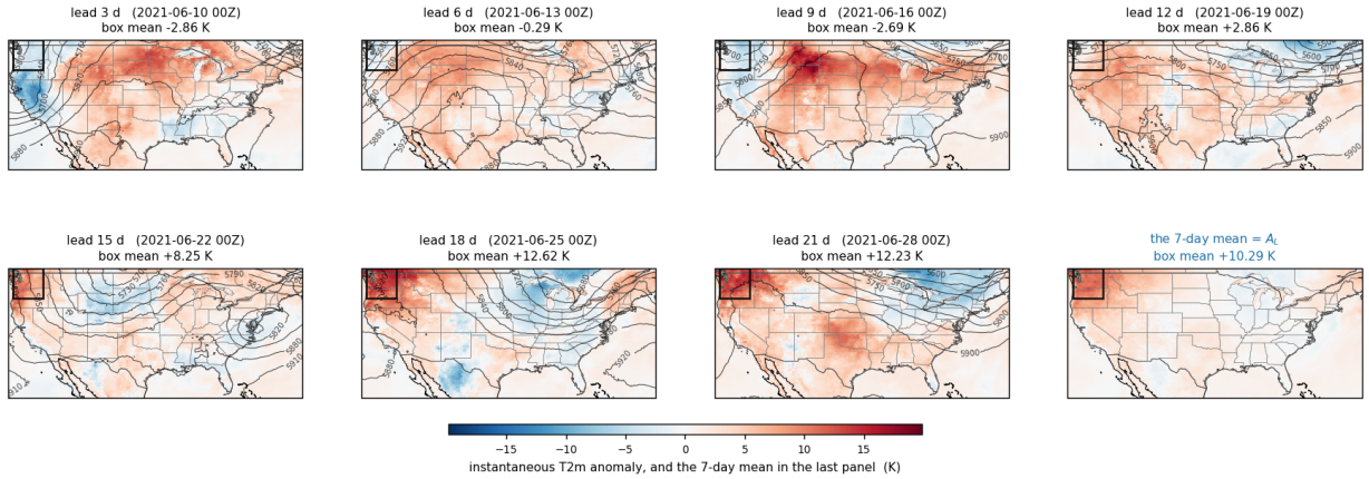
Figure 3: The single hottest surviving trajectory of the 2021 heat-dome run, followed from the 3-day checkpoint to the event, with the instantaneous temperature anomaly shaded and the upper-atmosphere pressure pattern contoured. At the 9-day checkpoint this trajectory had the fourth-coolest surface temperature of the 64 alive and would have ranked near the bottom on the conventional score. The scoring model ranked it tenth and gave it the maximum of eleven clones, because the ridge that later drives the heat dome was already building offshore while the surface beneath it had not yet warmed.
