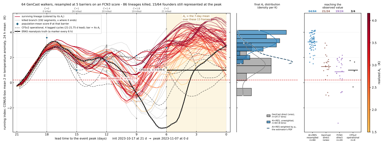
Figure A9: The CONUS-wide median week of November 2023, the second control. Observed +0.21 K, reached by all 64 trajectories, most extreme +4.16 K. Direct GenCast reaches it with 21 of 24 members, direct FourCastNet 3 with 19 of 24, and CFSv2 with 3 of 4 cycles. Every trajectory finished past the target, so the population was concentrated entirely beyond it and the weighted estimate carries no information about the event. This is the case referred to in Section 5, item 2.
