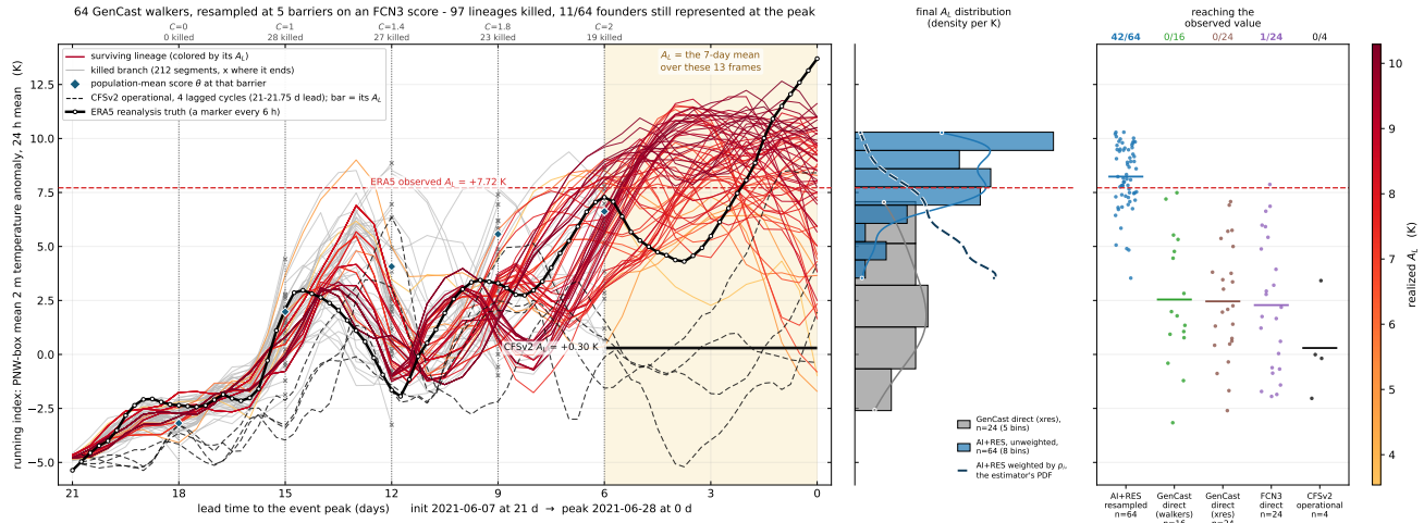
Figure A1: The 2021 Pacific Northwest heat dome, 64 trajectories, forecast from 21 days out. Left. Each line is one trajectory, plotted as its running regional temperature anomaly against time. Grey lines were discarded at a resampling step. Coloured lines survived to the event and are shaded by the value they reached. The dotted verticals are the five resampling steps, labelled by how hard the population was pushed and by how many trajectories were discarded. The blue diamonds are the population-average score. The shaded band on the right is the week the forecast is scored over. The black line with markers is the observed weather. The black dashed curves are the four CFSv2 operational cycles at the same lead, with their average drawn as a bar across the scored week. Middle. The distribution of final values for the 24-member direct GenCast ensemble in grey, for the AI+RES population in blue, and for the weighted estimate as a dashed line. Right. Where each method's members landed, with the number that reached the observed value printed above each column. Where a direct 24-member FourCastNet 3 ensemble was run it appears as a further column. Observed +7.72 K, reached by 42 of 64 trajectories, most extreme +10.29 K. The direct ensemble reaches it with none of 24 and stops at +7.08 K.
