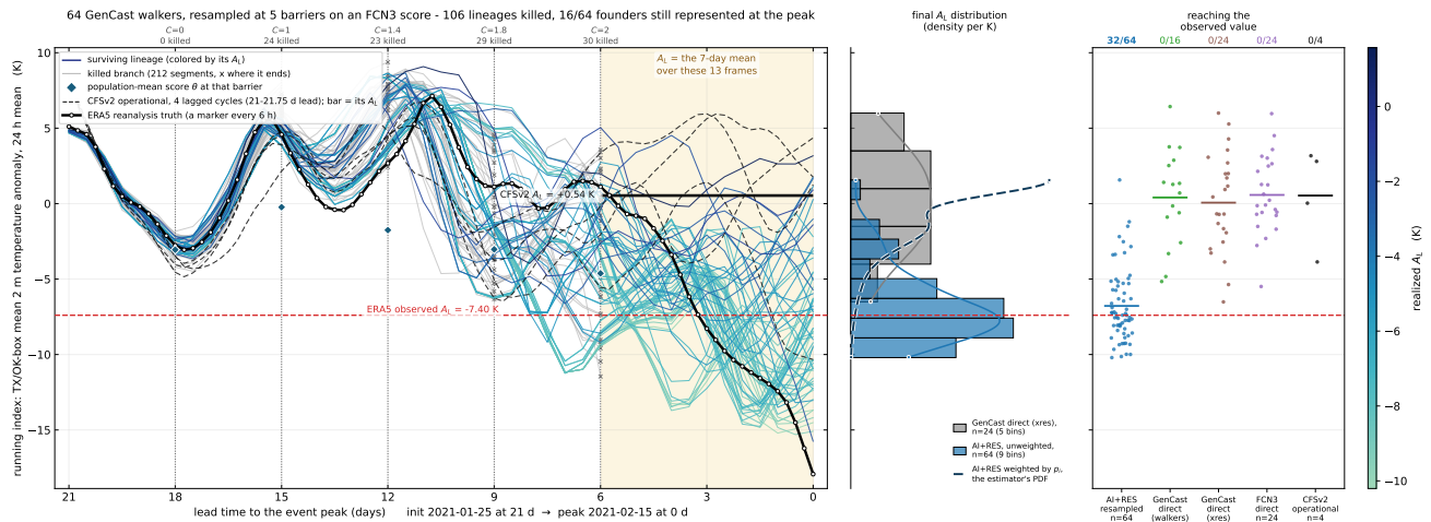
Figure A7: Winter Storm Uri, February 2021, over the Texas and Oklahoma region. The sign of the score is reversed for a cold event, so the method clones the coldest trajectories rather than the warmest. The schedule is otherwise the one used for the heat waves and was not retuned. Observed -7.40 K, reached by 32 of 64 trajectories, coldest -10.20 K. None of 24 direct GenCast members, 16 free-running trajectories or 24 direct FourCastNet 3 members reaches it.
