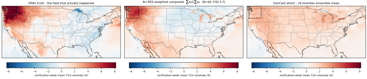
Figure 2: The 2021 Pacific Northwest heat dome, as maps of the week-average temperature anomaly. Left: the observed field. Middle: the AI+RES population three weeks out, with the dome in the observed location at the observed intensity. Right: the 24-member direct GenCast ensemble average from the same starting point, which contains no dome. The dashed box is the scored region. The middle panel is a weighted composite of trajectories selected for this event, so it shows where the method placed its samples and is not a forecast in the ordinary sense.
