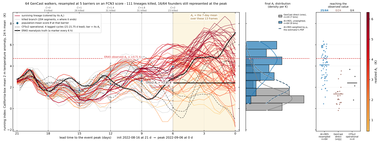
Figure A4: The September 2022 California heat wave. Observed +4.71 K, reached by 25 of 64 trajectories, most extreme +6.33 K. None of 24 direct GenCast members reaches it, the closest stopping at +4.70 K.
