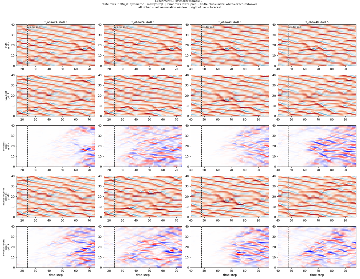
Figure 12: Experiment E: space-time (Hovmöller) diagnostics for one ensemble member (sample 0) of the Lorenz-96 sliding-window run. Columns are the four configurations (T_{\text{obs}}, \sigma_{\text{obs}}) \in \{24, 48\} \times \{0.0, 0.5\} ; the five rows are (1) truth, (2) SW-best reconstructed state, (3) SW-best signed error (prediction – truth), (4) invobs+hybrid (last-8) reconstructed state, and (5) invobs+hybrid signed error, with grid index k on the vertical axis and time step on the horizontal axis. State rows use a diverging colormap symmetric about \pm \max|\text{truth}| ; the two error rows share a scale set to the larger \max|\text{error}| across both methods within each column (blue = under-prediction, white = near-exact, red = over-prediction), making the two methods directly comparable. The dashed vertical line marks the window end T_{\text{obs}} : left of it is the last assimilation window, right of it the 50-step forecast. Both methods reproduce the truth’s travelling wave packets through and just past the window; the signed-error rows are near-white inside and immediately after the window and develop structured stripes as the chaotic forecast decorrelates, with SW-best showing visibly cleaner near-window error than the cold single-window invobs+hybrid at \sigma_{\text{obs}} = 0.5 . Forecast error growth far from the window is comparable across methods; this is a single illustrative member ( N = 50 overall), not a statistical summary.
