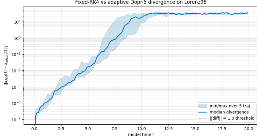
Figure 2: Fixed-step RK4 versus adaptive dopri5 integrator divergence on Lorenz-96. The vertical axis (log scale) is the L^2 state difference \|\mathbf{x}_{\text{RK4}}(t) - \mathbf{x}_{\text{adapt}}(t)\|_2 and the horizontal axis is model time t in MTU. The solid blue curve is the median over five warmed-up attractor states and the shaded band is the min/max envelope; the dashed grey line marks the order-one threshold. From identical initial conditions the two integrators agree to near machine precision while t \ll T_L , then the per-step truncation difference is amplified at the chaotic rate, crossing the order-one scale at a median t^* = 7.70 MTU (range [6.50, 8.30] ; 6.30 MTU for the single trajectory shown in the first panel) and saturating near 28.5 once the trajectories fully decorrelate. The takeaway is that t^* is the operational ceiling on assimilation-window length over which the two simulators represent the same physics; our single-window experiments use T = 1.0 MTU, comfortably inside it.
