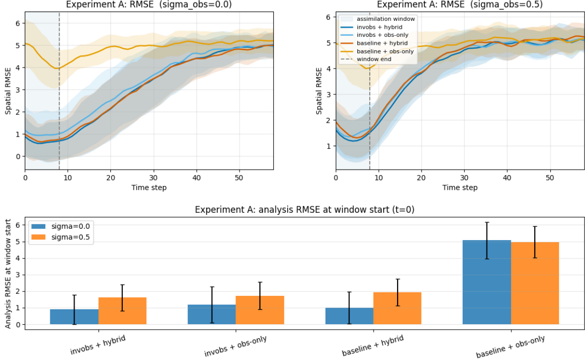
Figure 8: Experiment A: single 8-step assimilation window on Lorenz-96 ( N = 50 , \sigma_b = 1.0 ), comparing four initialization \times optimization combinations. Top row: ensemble-mean spatial RMSE versus time step for \sigma_{\text{obs}} = 0.0 (left) and \sigma_{\text{obs}} = 0.5 (right); the shaded band marks the assimilation window (steps 0–8), the dashed line the window end, and coloured envelopes are \pm 1 ensemble standard deviation. All curves fall to low error inside the window and then grow toward the climatological saturation (RMSE \approx 5 ) over the 50-step forecast, except baseline+obs-only, which never leaves the climatological level. Bottom: grouped bar chart of analysis RMSE at the window start ( t = 0 ). The three optimization-capable methods reach analysis RMSE \approx 1 at \sigma_{\text{obs}} = 0 and \approx 1.6 – 1.9 at \sigma_{\text{obs}} = 0.5 , while baseline+obs-only stays near 5. Physics-space (hybrid) warm-starting is essential to rescue the climatological-mean baseline from a poor observation-space local minimum; the best single-window choice is baseline+hybrid at \sigma_{\text{obs}} = 0 and invobs+hybrid at \sigma_{\text{obs}} = 0.5 , though their margin at \sigma_{\text{obs}} = 0 is within ensemble scatter.
