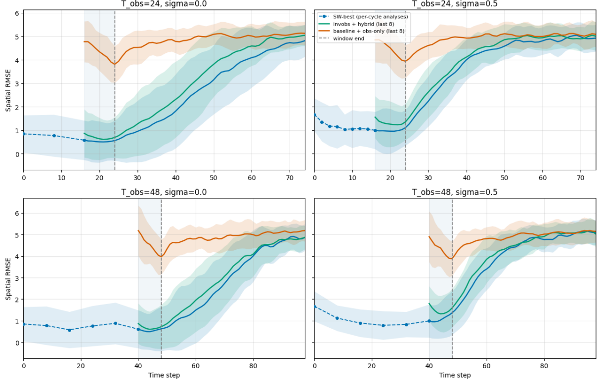
Figure 11: Experiment C (key comparison): sliding-window cycling versus single-window 4D-Var on Lorenz-96 ( N = 50 ). Each (T_{\text{obs}}, \sigma_{\text{obs}}) panel (rows T_{\text{obs}} = 24, 48 ; columns \sigma_{\text{obs}} = 0.0, 0.5 ) plots ensemble-mean spatial RMSE versus absolute time step with \pm 1 -std envelopes for three methods: SW-best (best-stride cycling with full observation history), a dashed per-cycle analysis-RMSE chain from t = 0 that hands off to a solid continuous curve for the last cycle plus 50-step forecast; invobs+hybrid on the last 8 observations; and baseline+obs-only on the last 8 observations. The shaded band is the last assimilation window [T_{\text{obs}} - 8, T_{\text{obs}}] and the dashed line marks the window end. baseline+obs-only stays near the climatological RMSE throughout the window; SW-best's chain descends as history accumulates, so it enters the last-window analysis time from a lower error than the cold single-window methods. The cycling advantage is most pronounced at \sigma_{\text{obs}} = 0.5 with long history T_{\text{obs}} = 48 , and marginal (curves overlap within N = 50 scatter) at \sigma_{\text{obs}} = 0 , where one well-posed 8-step window already pins the observed state. Deep in the chaotic forecast all methods converge to the same climatological saturation: cycling improves the analysis and short-lead forecast, not the Lyapunov-time-limited long-range predictability.
