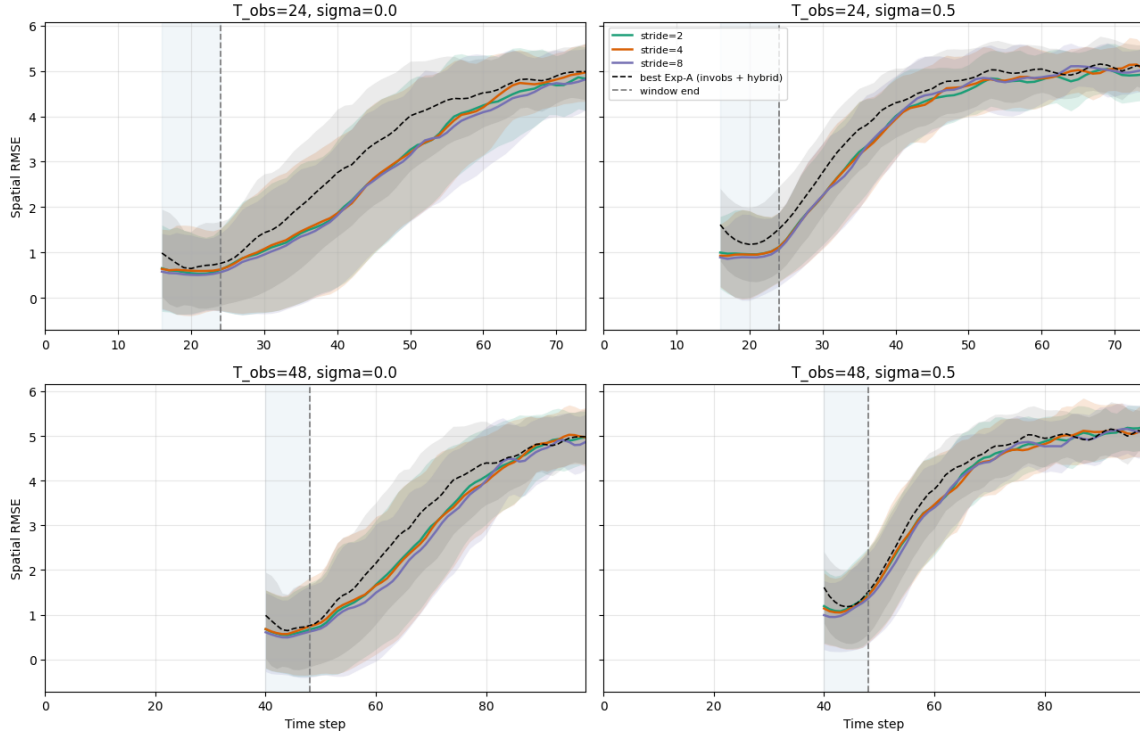
Figure 9: Experiment B1: sliding-window (cycling) 4D-Var stride sweep on Lorenz-96 ( N = 50 , invobs init each cycle, hybrid optimization, propagated-analysis background, cycling \sigma_b = 0.3 ). Each panel plots last-cycle ensemble-mean spatial RMSE versus absolute time step for strides 2, 4, 8 (coloured) with \pm 1 -std envelopes; rows are T_{\text{obs}} = 24 (top) and 48 (bottom), columns are \sigma_{\text{obs}} = 0.0 (left) and 0.5 (right). The shaded band is the last assimilation window [T_{\text{obs}} - 8, T_{\text{obs}}] and the dashed line is the window end; the dashed black curve is the best single-window Experiment-A method (baseline+hybrid at \sigma_{\text{obs}} = 0 , invobs+hybrid at \sigma_{\text{obs}} = 0.5 ), time-shifted so its window end coincides with the cycling runs. The three stride curves are nearly indistinguishable within ensemble scatter and all relax to climatological saturation; by mean forecast RMSE the selected best strides are 8, 2, 8, 8. Assimilation stride has little effect on Lorenz-96 cycling skill—differences are confined to the window and shortest lead times—so the best stride is a narrow tie-break rather than a strong preference.
