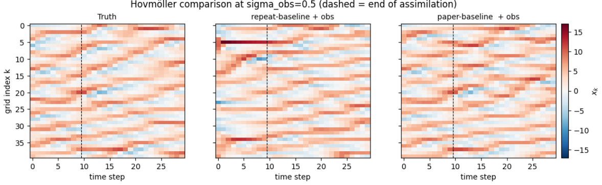
Figure 6: Hovmöller comparison of the two baselines at \sigma_{\text{obs}} = 0.5 . Each panel shows the Lorenz-96 state x_k (color, red–blue diverging scale) with grid index k on the vertical axis and time step on the horizontal axis: ground-truth trajectory (left), observation-space 4D-Var initialized from the repeat-interleave baseline (center), and from the climatological-mean baseline (right). The dashed vertical line marks the end of the 10-step assimilation window; everything to its right is free forecast. The repeat baseline carries visible artifacts and a distorted wave pattern out of the window, whereas the climatological-mean baseline reproduces the truth’s traveling-wave structure more faithfully into the forecast under moderate observation noise.
