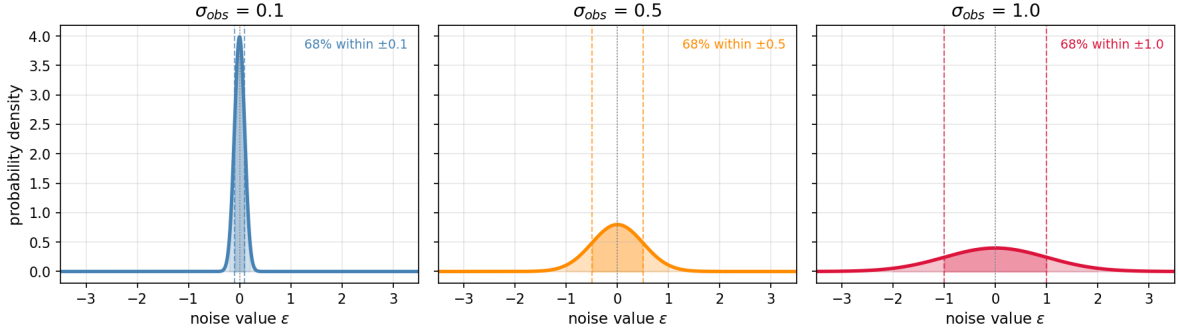
Figure 1: Gaussian observation-noise probability density functions used to corrupt the observations in every experiment. Each curve is the density of \varepsilon \sim \mathcal{N}(0, \sigma_{\text{obs}}^2) for one of the three noise standard deviations \sigma_{\text{obs}} \in \{0.1, 0.5, 1.0\} ; the horizontal axis is the noise value added to a single observed component and the vertical axis is the probability density. Each observed site and time receives an independent draw, so the observation-error covariance is \mathbf{R} = \sigma_{\text{obs}}^2 \mathbf{I} . The \sigma_{\text{obs}} = 0.1 case is a sharp, nearly-clean perturbation, whereas \sigma_{\text{obs}} = 1.0 broadens to a level comparable to the Lorenz-96 state amplitude, making observations substantially less informative and stress-testing the assimilation methods.
