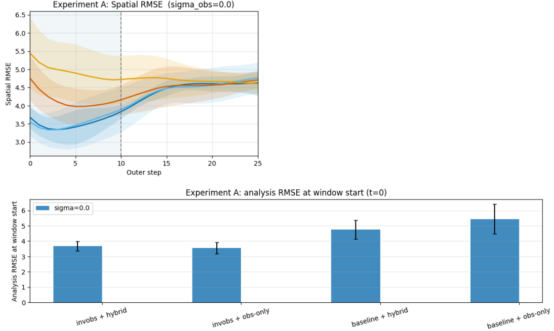
Figure 15: Kolmogorov Experiment A: a single 10-step assimilation window ( T_{\text{obs}} = \text{WINDOW\_T} = 10 , \sigma_b = 1.0 , \sigma_{\text{obs}} = 0.0 ), comparing the four initialization \times optimization combinations. Top: ensemble-mean spatial RMSE ( \pm 1 standard deviation over the N = 8 ensemble) versus outer step, spanning the assimilation window (shaded, 0–10, dashed window-end line) and the free forecast to step 25. Bottom: bar chart of analysis RMSE at the window start ( t = 0 ). The invobs combinations reach lower in-window RMSE ( \approx 3.5 – 3.7 ) than the baseline combinations ( \approx 4.8 – 5.5 ), but all curves converge toward saturation once the forecast leaves the window, reflecting the chaotic flow and extreme observation sparsity (16 of 4096 points). The final L-BFGS costs are invobs+hybrid 56,385 and invobs+obs-only 45,760 versus baseline+hybrid 168,341 and baseline+obs-only 138,254: invobs initialization places the optimizer in a basin roughly 3\times lower in cost and yields the best in-window analyses, though forecast skill saturates after the window.
