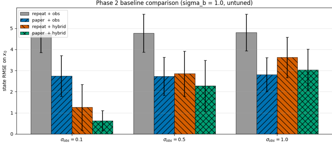
Figure 5: Analysis RMSE comparison of the two baseline initializations under untuned full 4D-Var ( \sigma_b = 1.0 fixed). Grouped bars show post-assimilation state RMSE on x_0 ( \pm one standard deviation over N = 100 trajectories) for the four combinations of initializer (repeat-interleave vs. climatological-mean) and optimization mode (observation-space vs. hybrid), across noise levels \sigma_{\text{obs}} \in \{0.1, 0.5, 1.0\} . The repeat-interleave baseline with observation-only optimization (grey) is worst at every noise level; replacing it with the climatological-mean baseline and, especially, adding hybrid optimization lowers RMSE substantially (the climatological+hybrid bars are lowest, most clearly at \sigma_{\text{obs}} = 0.1 ). A better cold-start prior and hybrid optimization each reduce analysis error even before the background weight \sigma_b is tuned, motivating the per-cell \sigma_b sweep that follows. (Direct x_0 RMSE of the raw initializers at \sigma_{\text{obs}} = 0 is 4.78 for repeat vs. 3.09 for climatological mean, ratio 0.646.)
