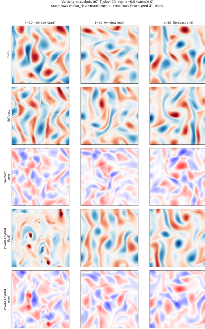
Figure 18: Kolmogorov vorticity-field snapshot comparison for Experiment C at T_{\text{obs}} = 20 , \sigma_{\text{obs}} = 0.0 (ensemble sample 0). The 5 \times 3 grid has columns at three times relative to the last-window start: window start ( t = 10 ), window end ( t = 20 ), and forecast end ( t = 35 ). Rows top to bottom: ground-truth vorticity; the sliding-window-best prediction; the sliding-window-best signed error; the single-window invobs+hybrid prediction; and the invobs+hybrid signed error. State rows use a diverging red–blue colormap (RdBu_r) scaled to \pm \max |\text{truth}| ; the two error rows share a single symmetric blue–white–red scale (bwr) showing prediction minus truth. At window start both methods reproduce the large-scale structures with small error, but by forecast end the error fields grow to the magnitude of the state itself. Both methods track the turbulent field while observations constrain it, but errors saturate at the state scale by forecast end, visually corroborating the RMSE saturation and the difficulty of reconstructing a 64 \times 64 turbulent field from 16 point observations.
