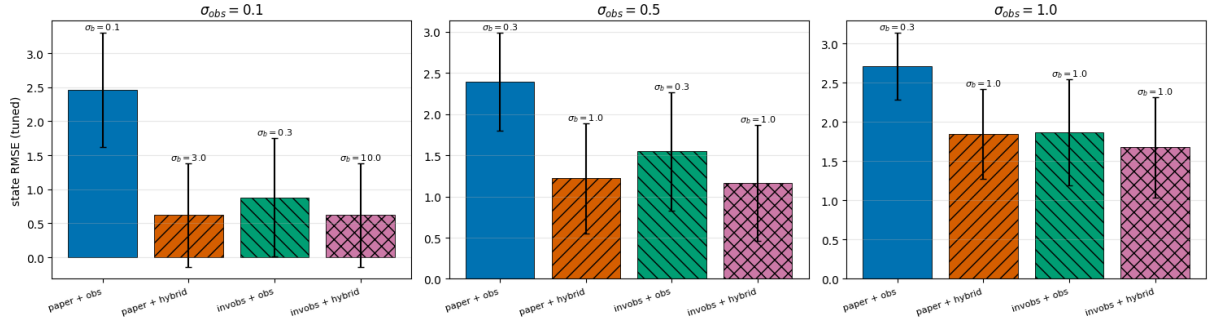
Figure 7: KEY RESULT —tuned- \sigma_b full 4D-Var on Lorenz-96. One panel per observation-noise level ( \sigma_{\text{obs}} = 0.1, 0.5, 1.0 , left to right); within each panel the four bars are the (initializer \times optimization-mode) combinations paper+obs, paper+hybrid, invobs+obs, invobs+hybrid, showing the lowest analysis RMSE on \mathbf{x}_0 ( \pm one standard deviation, N = 16 ) after sweeping \sigma_b \in \{0.1, 0.3, 1.0, 3.0, 10.0\} ; the optimal \sigma_b is annotated above each bar. The learned-inverse initialization with hybrid optimization (rightmost bar) attains the lowest RMSE at every noise level (0.620, 1.168, 1.676), and hybrid optimization dramatically improves the climatological-mean baseline over observation-only (paper+obs 2.393 \rightarrow paper+hybrid 1.223 at \sigma_{\text{obs}} = 0.5 ). The annotated optimal \sigma_b values reveal an honest negative result: the expected ordering “invobs+hybrid prefers a smaller \sigma_b than paper+obs” does not hold (invobs+hybrid selects \sigma_b = 10.0/1.0/1.0 versus paper+obs 0.1/0.3/0.3), and tuning \sigma_b helps only marginally over the untuned \sigma_b = 1 in most cells.
