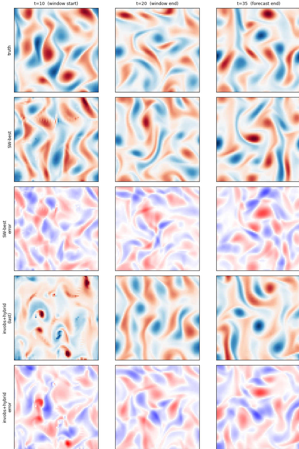
Figure 18: Kolmogorov vorticity-field snapshot comparison for Experiment C at T_{\text{obs}} = 20 , \sigma_{\text{obs}} = 0.0 (ensemble sample 0). The 5 \times 3 grid has columns at three times relative to the last-window start: window start ( t = 10 ), window end ( t = 20 ), and forecast end ( t = 35 ). Rows top to bottom: ground-truth vorticity; the sliding-window-best prediction; the sliding-window-best signed error; the single-window invobs+hybrid prediction; and the invobs+hybrid signed error. State rows use
