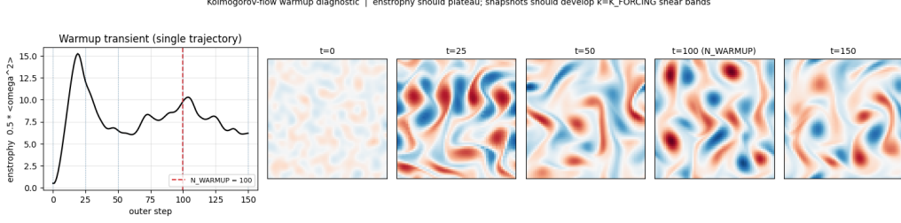
Figure 14: Warmup and stationarity diagnostic for the Kolmogorov-flow spin-up, on a single trajectory. Left: entrophy \frac{1}{2}\langle\omega^2\rangle versus outer integration step; the red dashed line marks the warmup length N_{\text{warmup}} = 100 . Entrophy starts at 0.500 from the smooth filtered cold start, overshoots to a peak near 15.3 around step 20, then relaxes to 9.824 at t = 100 and 6.195 at t = 150 . The remaining panels show vorticity snapshots (RdBu_r, shared scale) at t = 0, 25, 50, 100, 150 , evolving from a featureless field into developed k = 4 turbulent shear bands. The last-20-step relative drift is 10.82%, marginally above the \lesssim 10\% heuristic, so the flow is reported as approximately quasi-stationary. Integrating 100 warmup steps brings the cold start into a turbulent, approximately stationary regime suitable for generating assimilation experiments.
