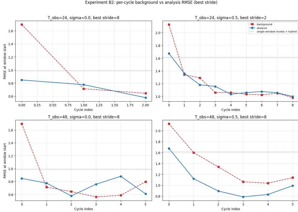
Figure 10: Experiment B2: per-cycle error reduction for the best-stride sliding-window run in each (T_{\text{obs}}, \sigma_{\text{obs}}) configuration ( N = 50 ). Each panel plots ensemble-mean spatial RMSE at the window-start time versus cycle index for the J_b background (red dashed squares, the previous analysis propagated to the new window) and the analysis (blue circles), with the single-window invobs+hybrid analysis RMSE as a dotted horizontal reference. Panels: T_{\text{obs}} = 24 best stride 8 ( \sigma_{\text{obs}} = 0 , 3 cycles) and 2 ( \sigma_{\text{obs}} = 0.5 , 9 cycles); T_{\text{obs}} = 48 best stride 8 for both noise levels (6 cycles). The analysis lies at or below the background within each cycle, and after cycle 0 the cycled analysis drops below the single-window reference. The descent is cleanest at \sigma_{\text{obs}} = 0.5 ; at \sigma_{\text{obs}} = 0 the curves are noisier and non-monotone because a single 8-step window already over-determines the 10 observed components, leaving N = 50 sampling noise dominant. Cycling reduces background error into a better analysis each cycle, most clearly when observations are noisy.
