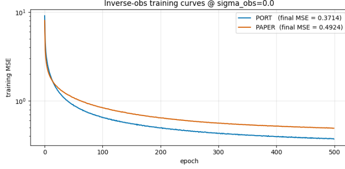
Figure 4: Training-loss curves for the two inverse observation operators at \sigma_{\text{obs}} = 0 . Both networks are trained on the same 32,000-trajectory dataset with identical Adam settings (500 epochs); vertical axis: training MSE (log scale); horizontal axis: epoch. The blue curve is the original PyTorch port (GELU activations, flat width-32 residual stack, bilinear upsampling), converging to final MSE 0.3714; the orange curve is the paper-faithful inverter (SiLU activations, 128 \rightarrow 64 \rightarrow 32 \rightarrow 16 channels, BN after every convolution, cubic-periodic upsampling, no skip connections), converging to 0.4924. The two curves track closely, and despite the architectural differences the paper-faithful inverter reproduces the port’s reconstruction quality (held-out test L_1 ratio 1.165, within the 30% acceptance band).
