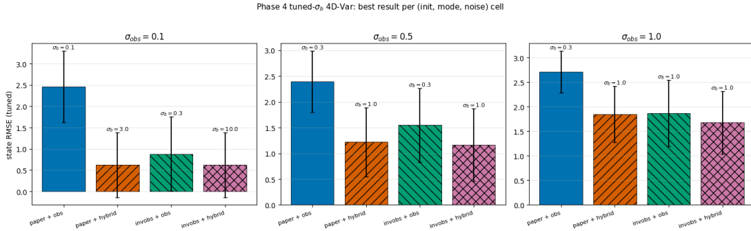
Figure 7: KEY RESULT—tuned- \sigma_b full 4D-Var on Lorenz-96. One panel per observation-noise level ( \sigma_{\text{obs}} = 0.1, 0.5, 1.0 , left to right); within each panel the four bars are the (initializer \times optimization-mode) combinations paper+obs, paper+hybrid, invobs+obs, invobs+hybrid, showing the lowest analysis RMSE on \mathbf{x}_0 ( \pm one standard deviation, N = 16 ) after sweeping \sigma_b \in \{0.1, 0.3, 1.0, 3.0, 10.0\} ; the optimal \sigma_b is annotated above each bar. The learned-inverse initialization with hybrid optimization (rightmost bar) attains the lowest RMSE at every noise level (0.620, 1.168, 1.676), and hybrid optimization dramatically improves the climatological-mean baseline over observation-only (paper+obs 2.393 \rightarrow paper+hybrid 1.223 at \sigma_{\text{obs}} = 0.5 ). The annotated optimal \sigma_b values also show the honest negative result discussed in the text: invobs+hybrid selects \sigma_b = 10.0/1.0/1.0 versus paper+obs 0.1/0.3/0.3, the opposite of the expected ordering.
