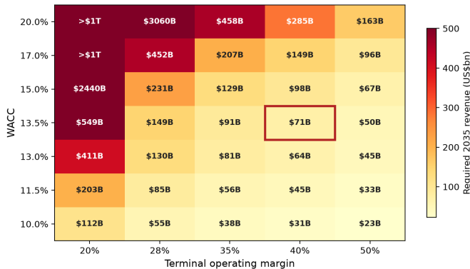
Reverse-DCF sensitivity: 2035 revenue needed to justify US$62bn equity (red box = base-case WACC 13.5% / terminal margin 40%)
