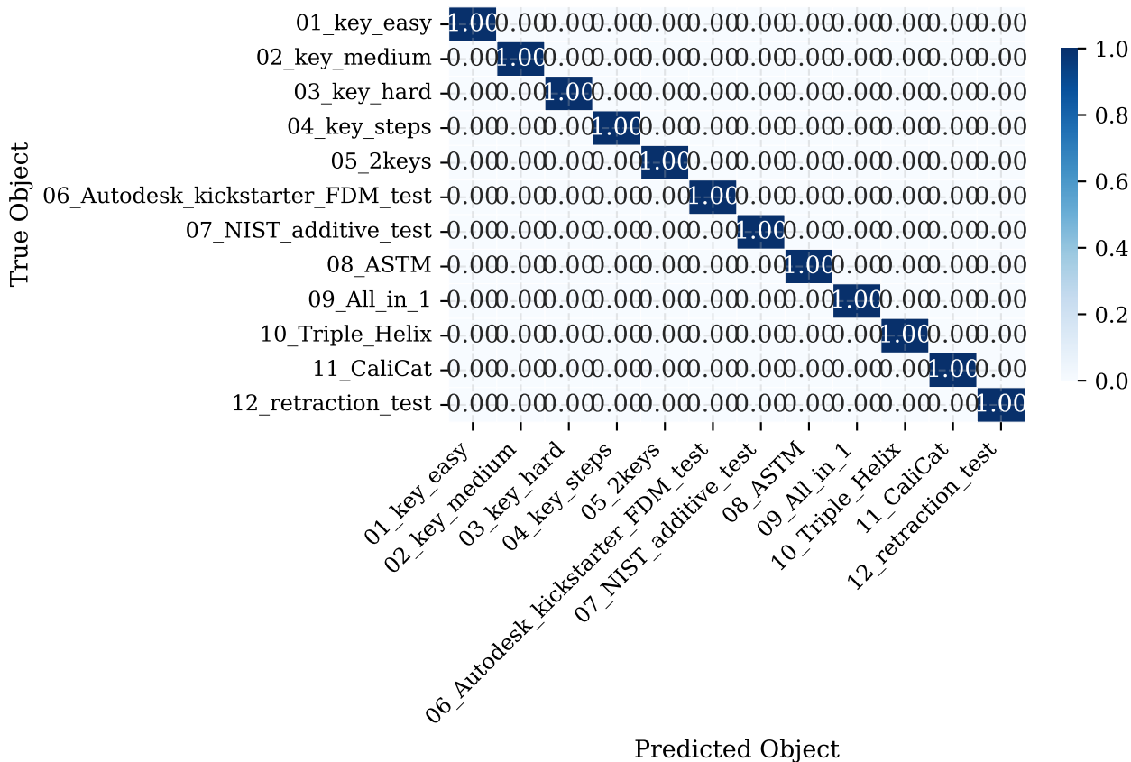
Figure 4. Confusion Matrix: Fused Attack (Post-Defense)
