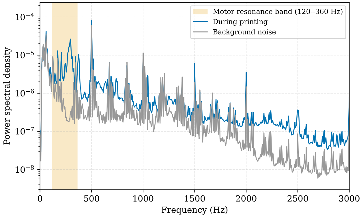
Motor band elevated +4.92 dB during printing
