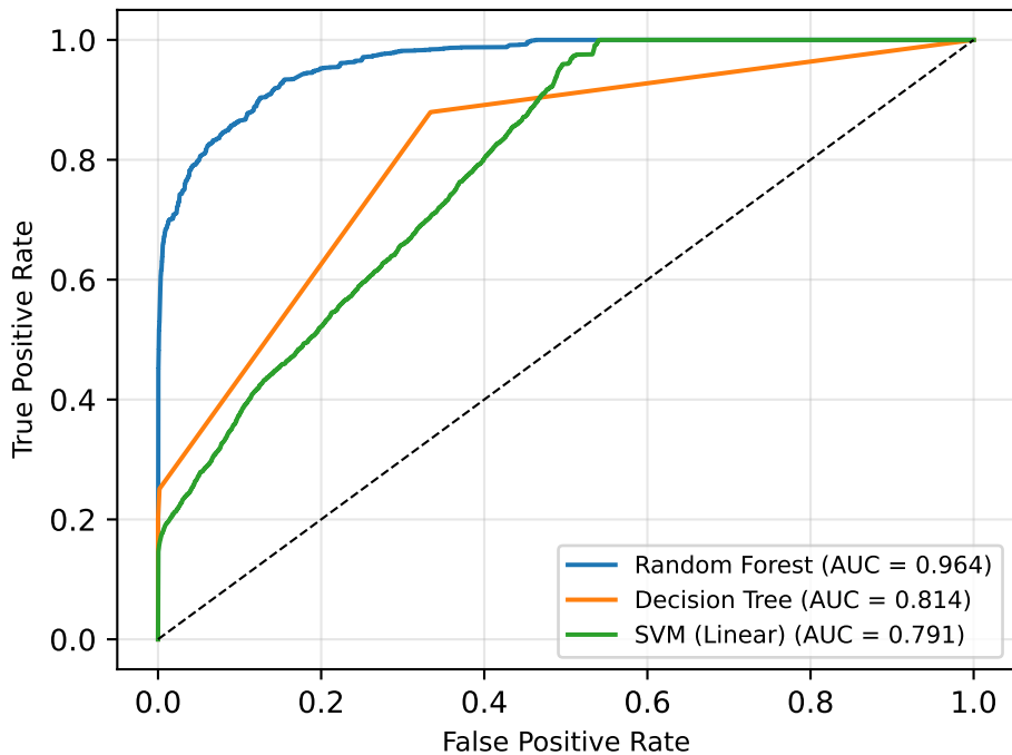
ROC Curves - HAI 22.04 Real ICS Data
