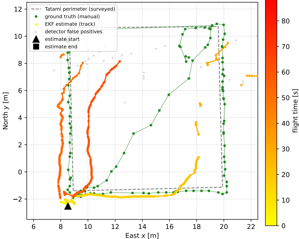
Estimated track vs. ground truth (raw filter output)
