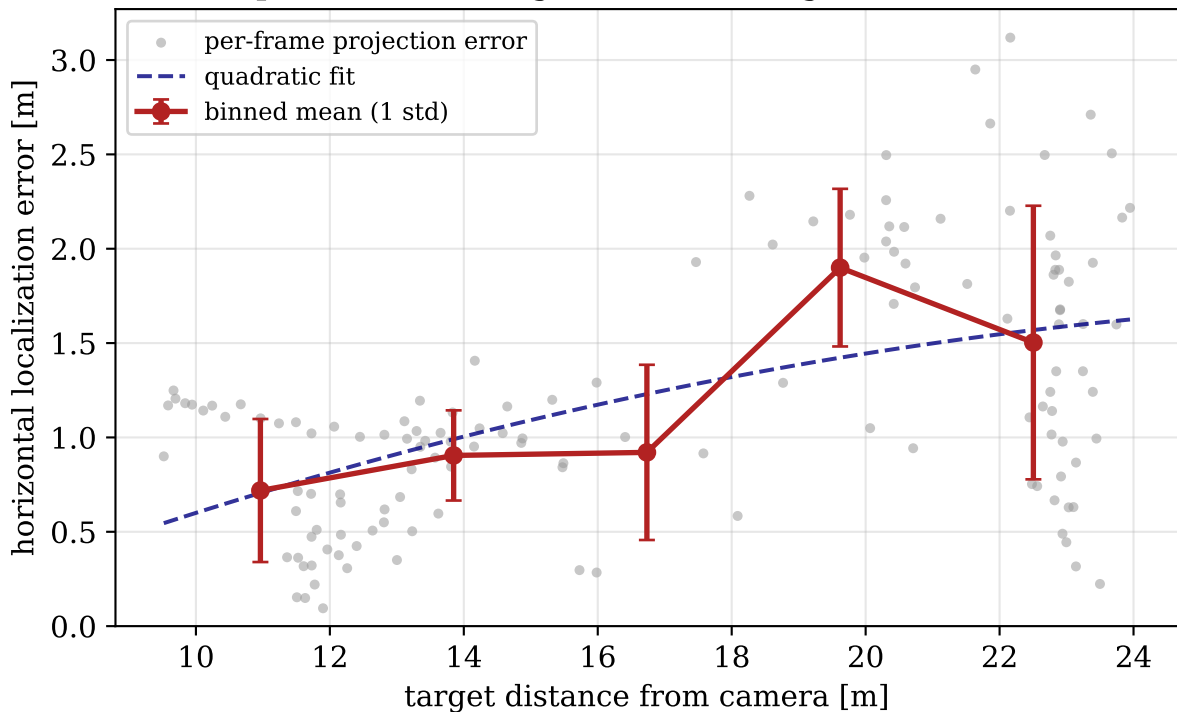
Ground-plane lift error grows with range (correlation 0.53)
