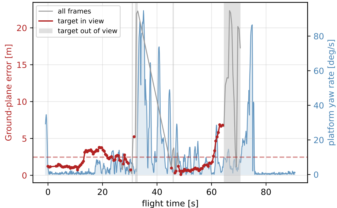
(a) Error vs. platform rotation (RMSE 2.46 m in view, 6.27 m overall)
