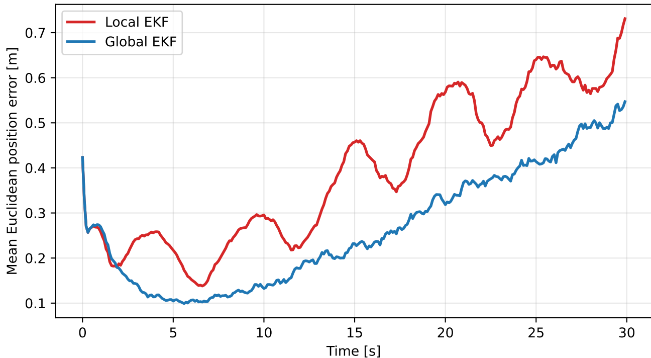
Anisotropic inertial-frame process noise: global frame is superior
