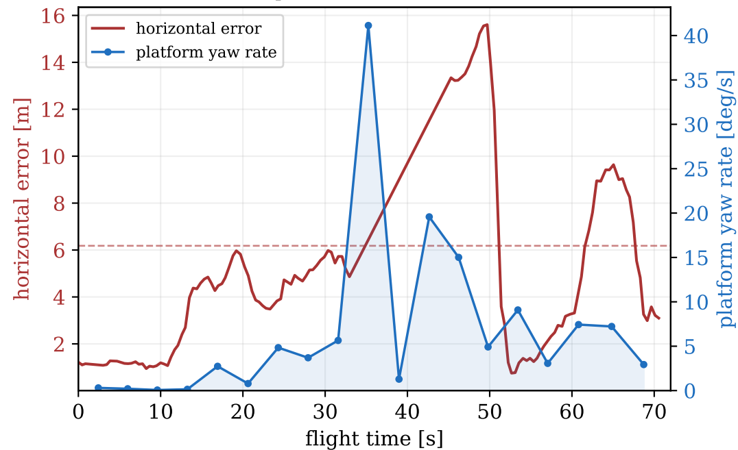
(a) Error vs. platform rotation (RMSE 6.18 m)
