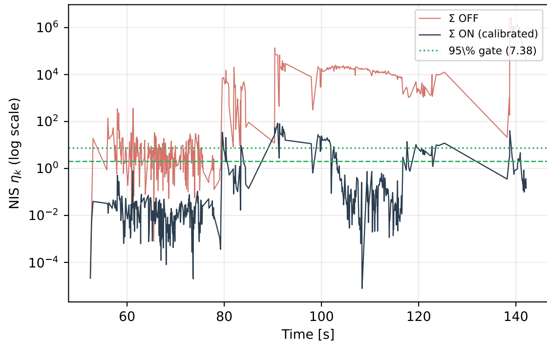
(b) NIS over the flight
