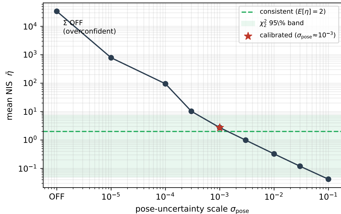
(a) Filter consistency vs. pose-uncertainty propagation
