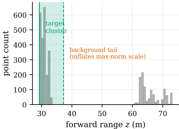
(b) Range histogram in frustum
