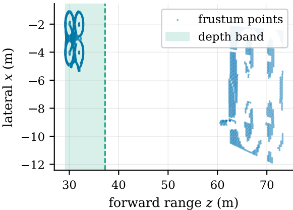
(a) Frustum point cloud (top view)
