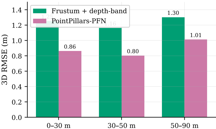
3D localization error vs. range
