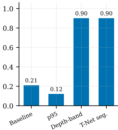
Detection precision ↑
