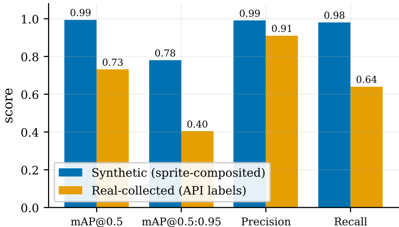
2D detector (YOLOv11s) performance
