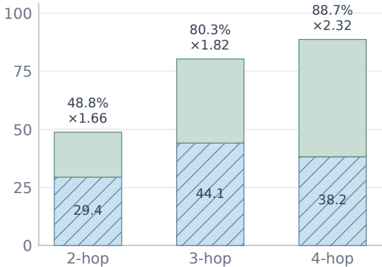
Groups with a within-group ordering (%)
