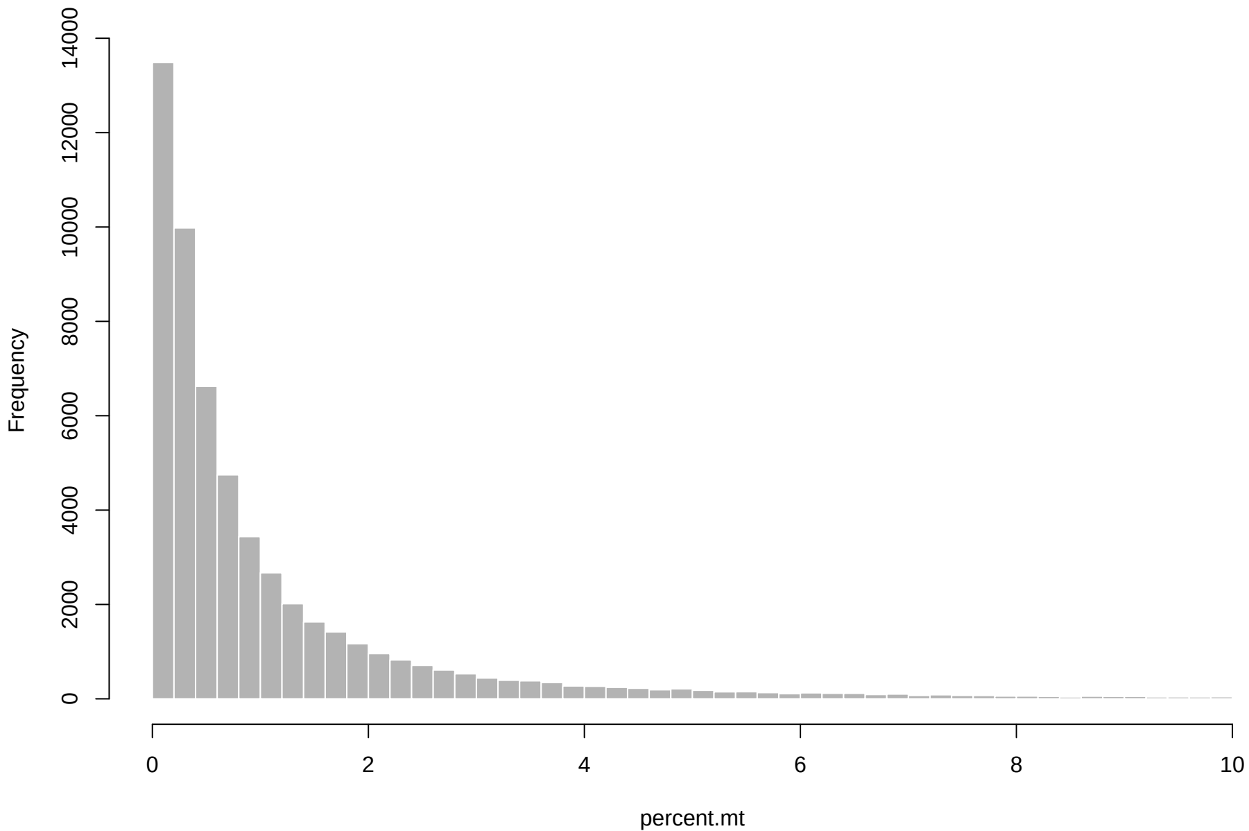
immune analytic-cohort percent.mt
