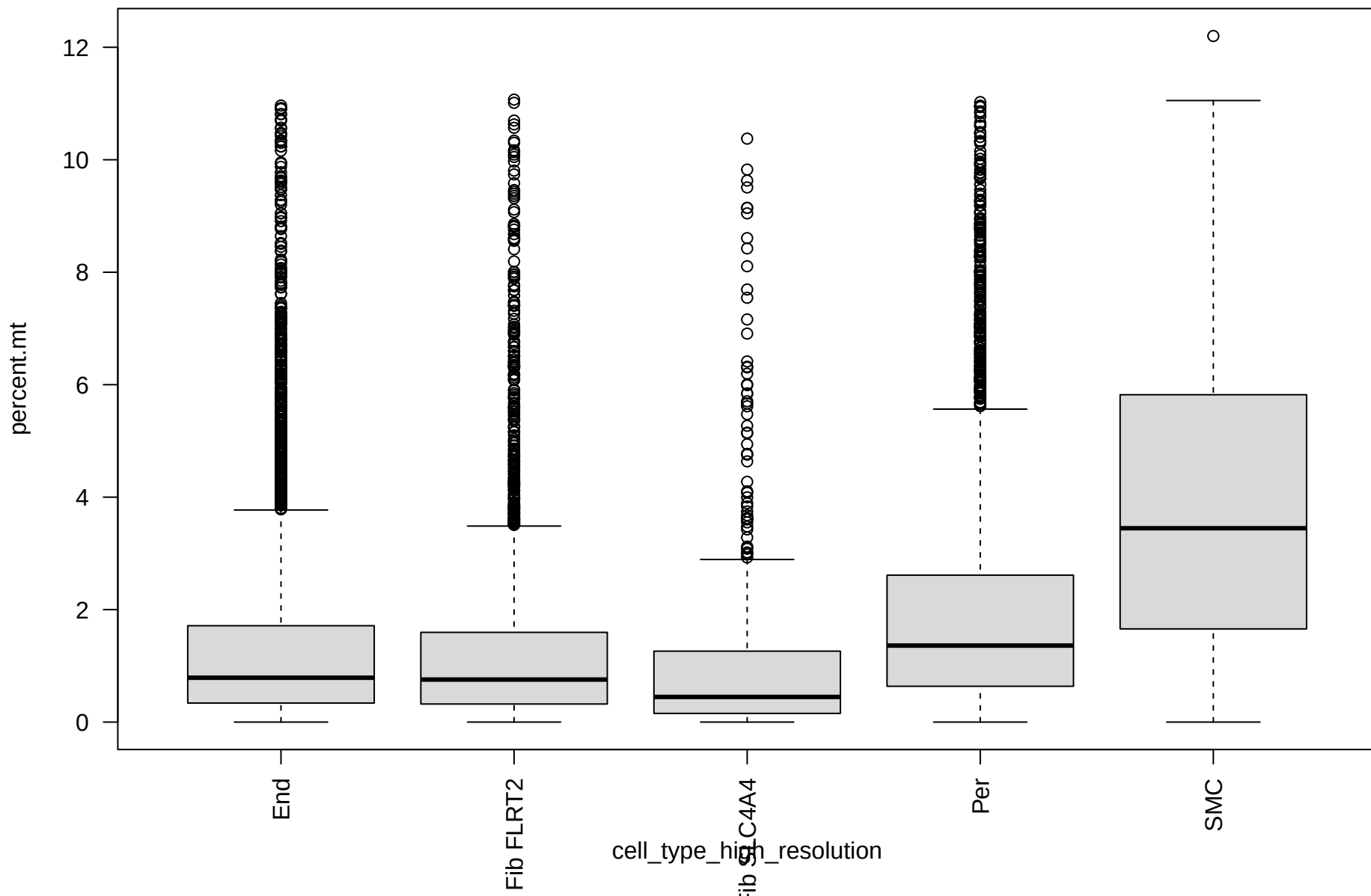
percent.mt by fine cell type
