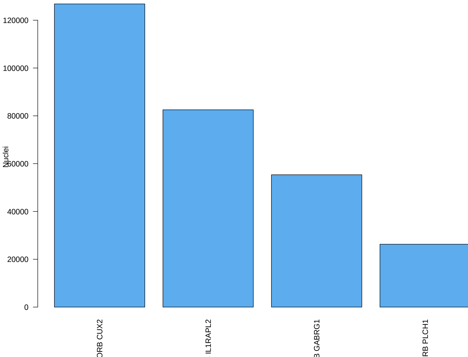
Analytic nuclei by fine cell type
